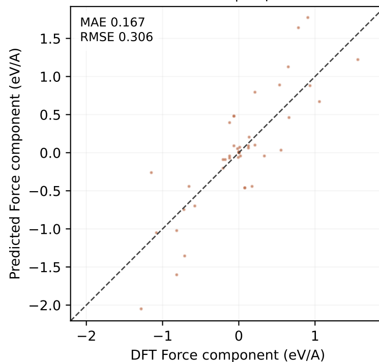
MatPES test | 78 points
