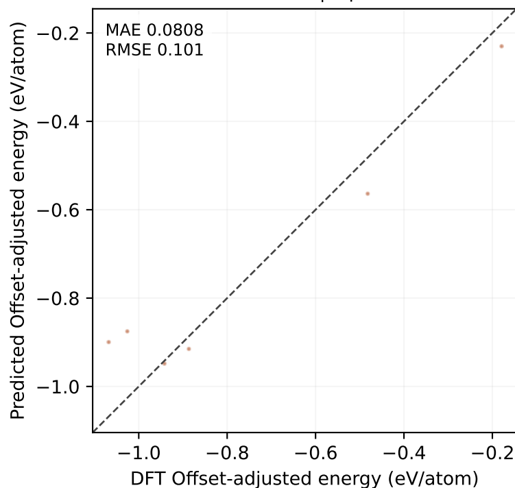
MatPES test | 6 points
