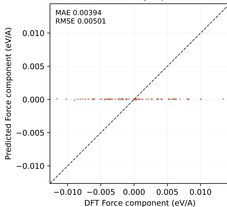
MatPES test | 87 points
