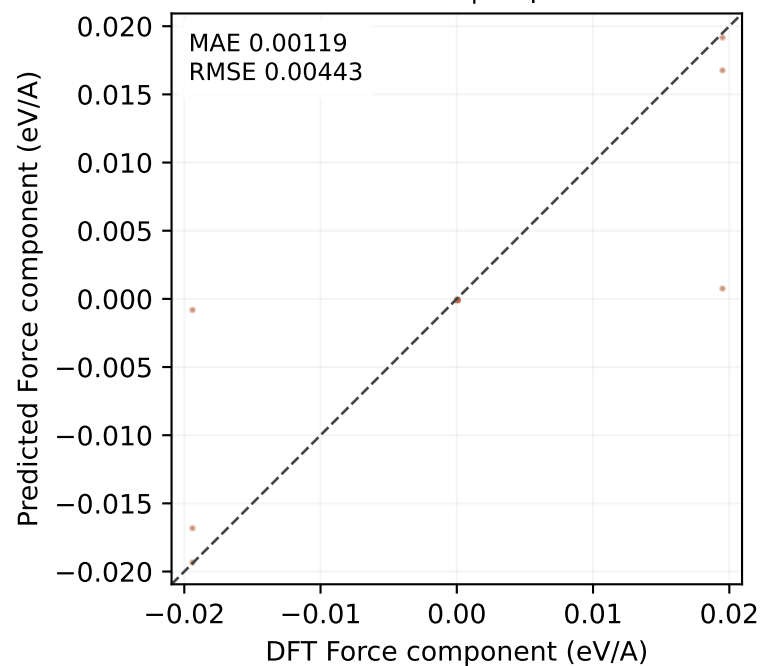
MatPES test | 36 points
