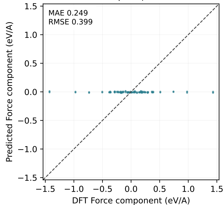
MatPES test | 36 points
