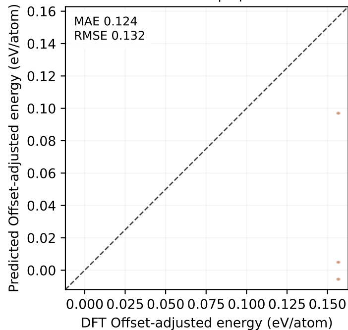
MatPES test | 3 points
