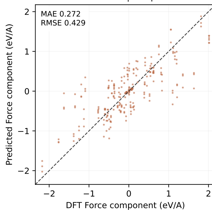
MP-ALOE test | 2,079 points
