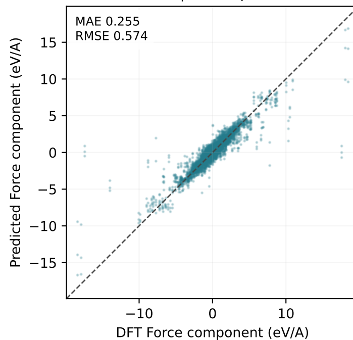
MatPES test | 342 points
