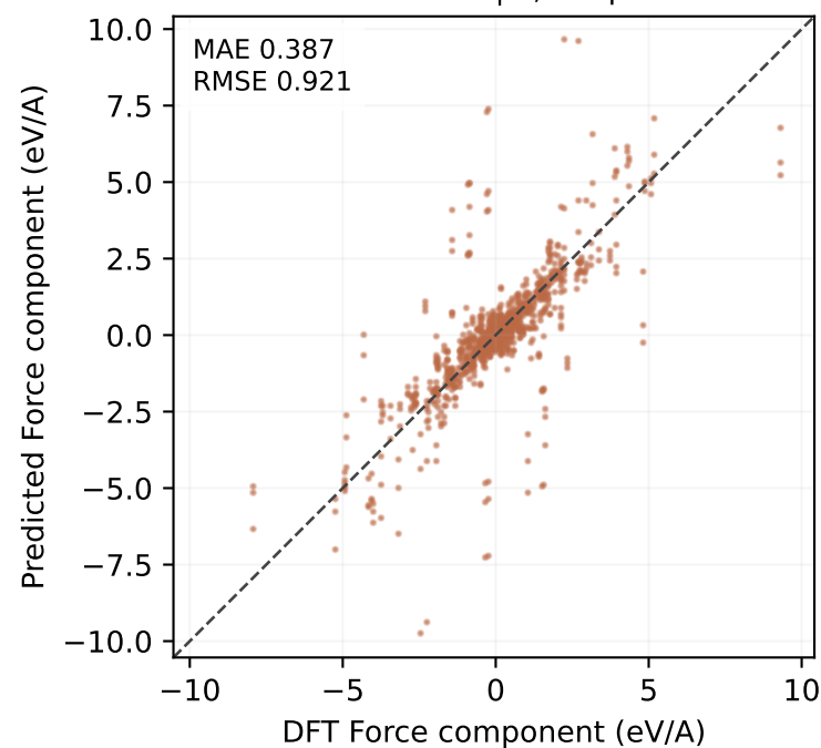
MP-ALOE test | 2,079 points
