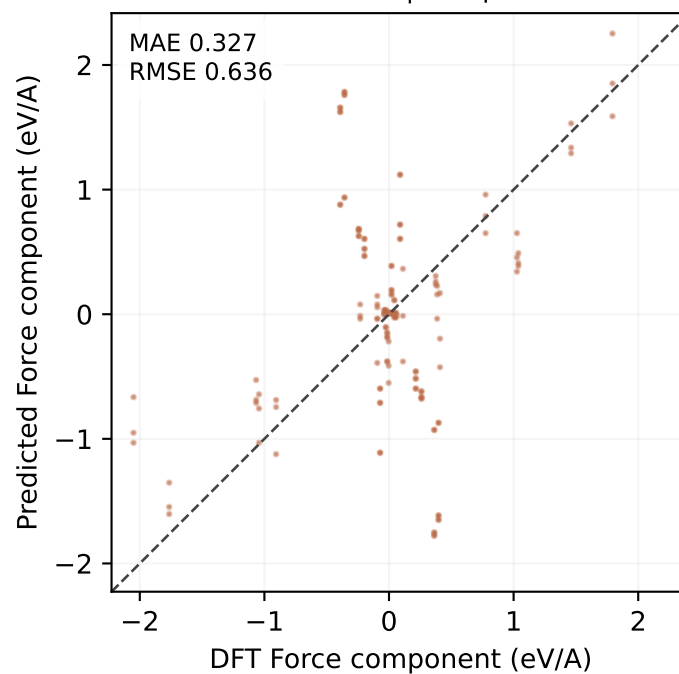
MP-ALOE test | 1,620 points
