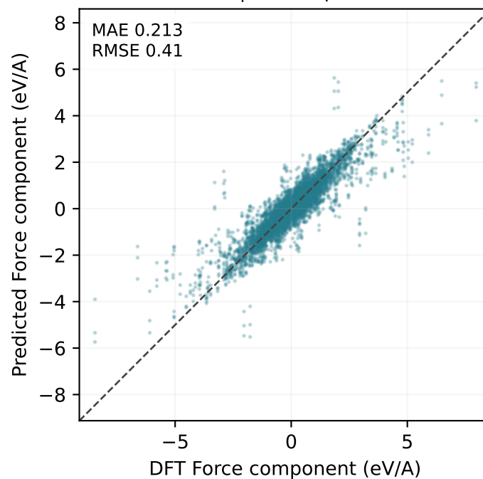
MatPES test | 288 points
