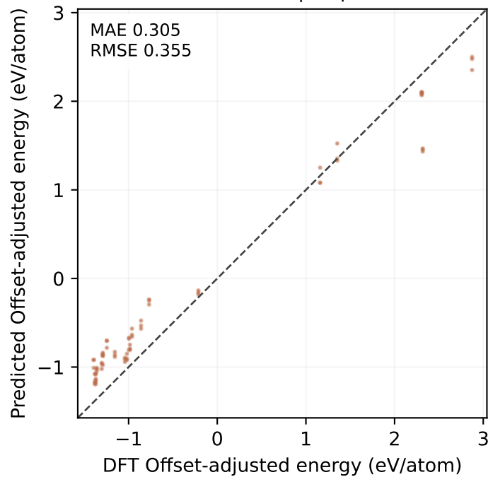
MP-ALOE test | 72 points
