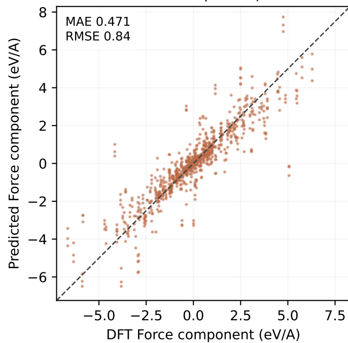
MP-ALOE test | 1,134 points
