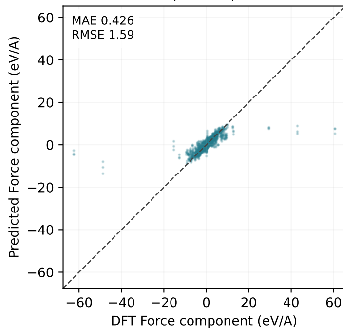
MatPES test | 3,456 points
