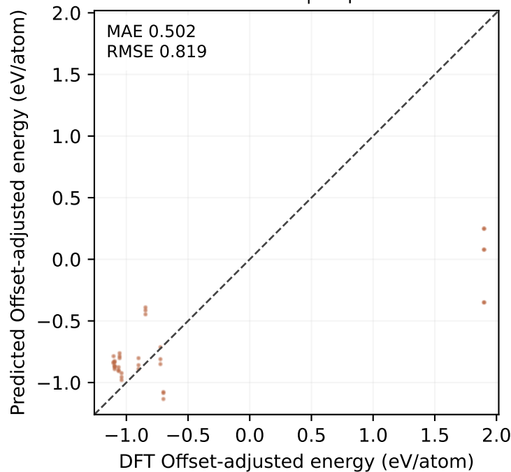
MP-ALOE test | 117 points
