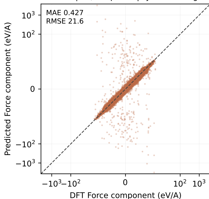
Molten test | 47,700 points | symmetric-log axes
