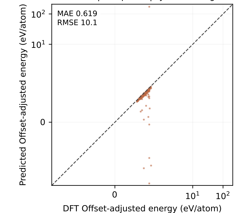
Molten test | 300 points | symmetric-log axes
