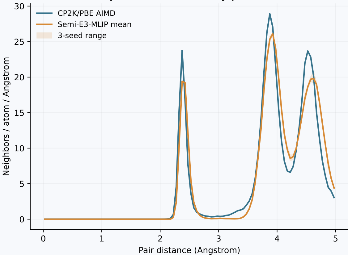
Slab pair-distance density | 100-500 fs
