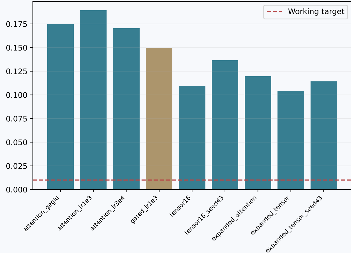
Validation energy MAE (eV/atom)
