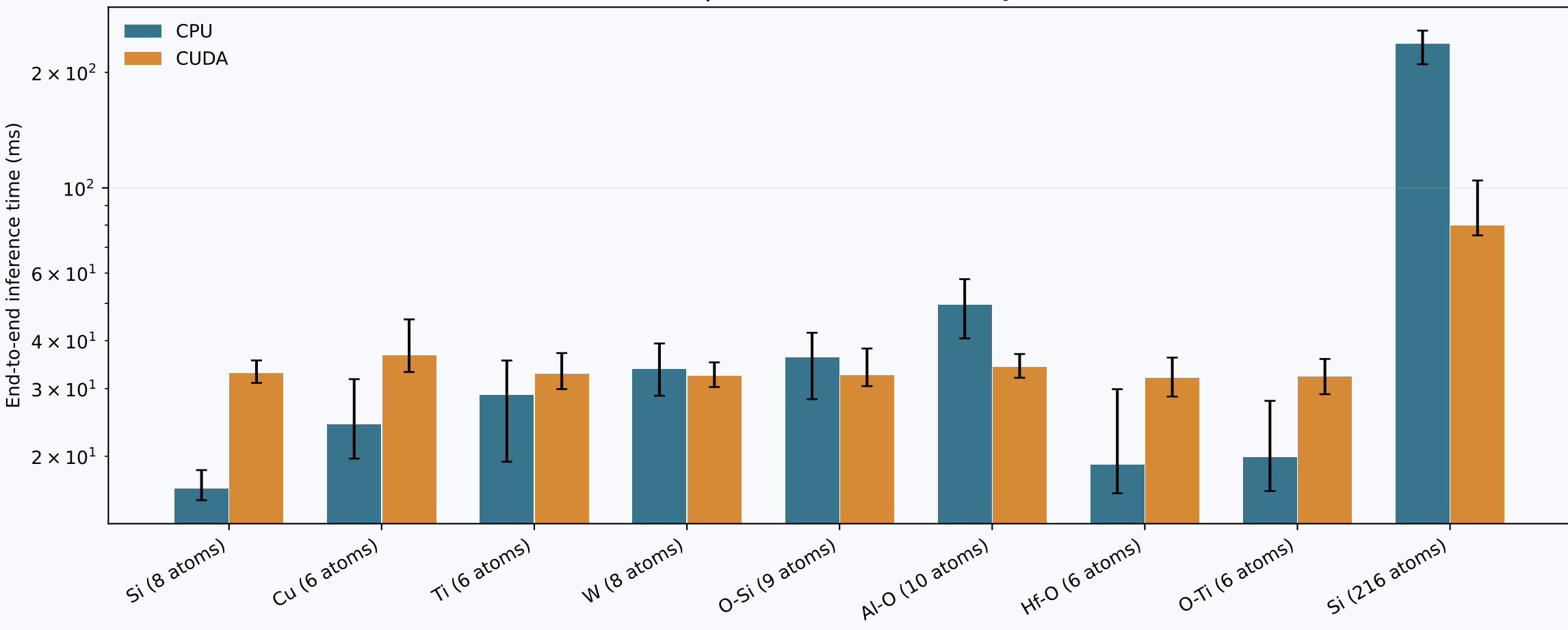
Local inference cost | median and 10th-90th percentile interval
