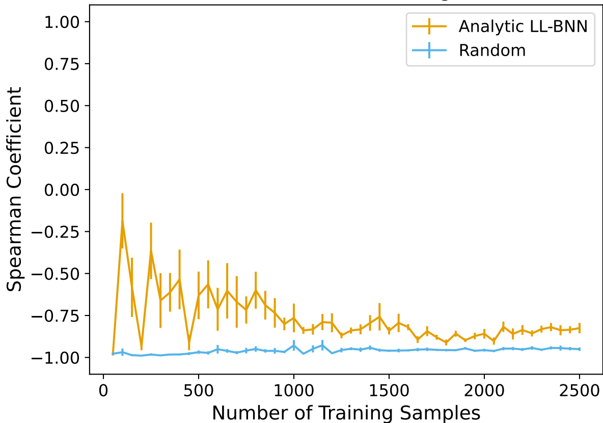
Correlation over Active Learning Iterations
