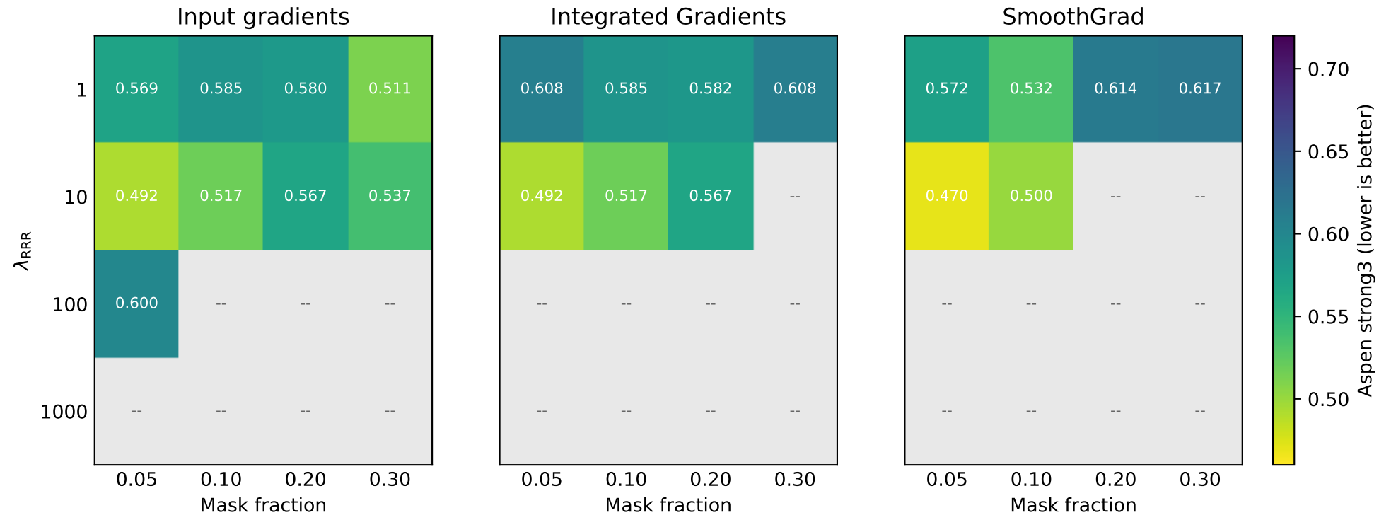
Best Aspen strong3 by completed hyperparameter cell
