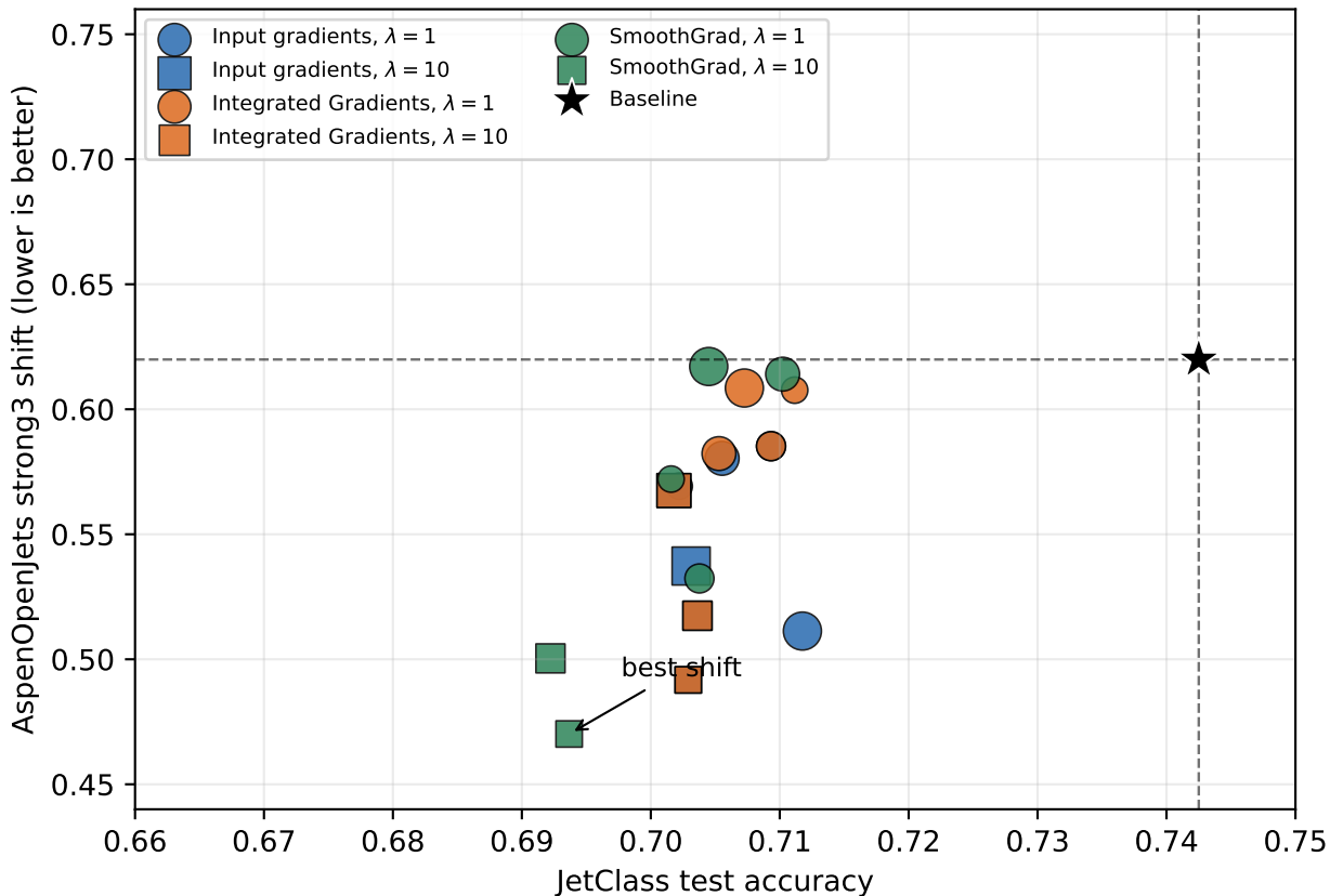
Completed RRR sweep: in-domain accuracy vs. target-domain shift
