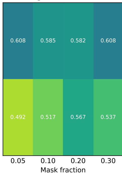
Integrated Gradients
