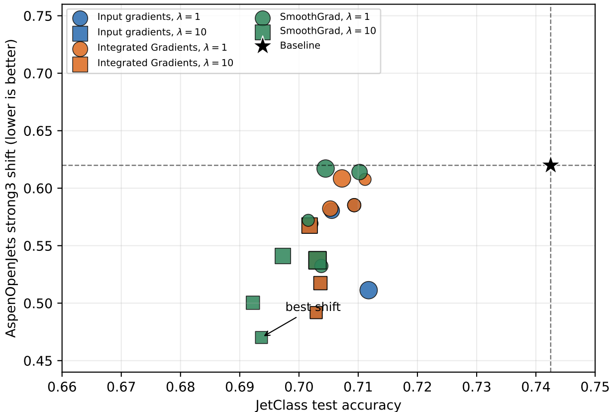
Focused RRR sweep: in-domain accuracy vs. target-domain shift
