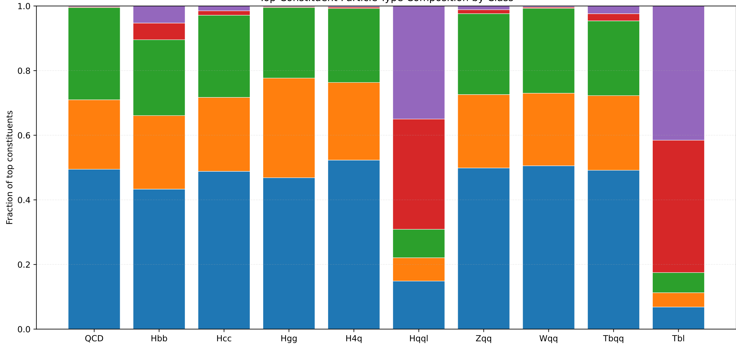
Top-Constituent Particle-Type Composition by Class
