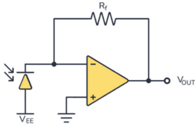
Figure 3.13 Photodiode Light Sensing Circuit
