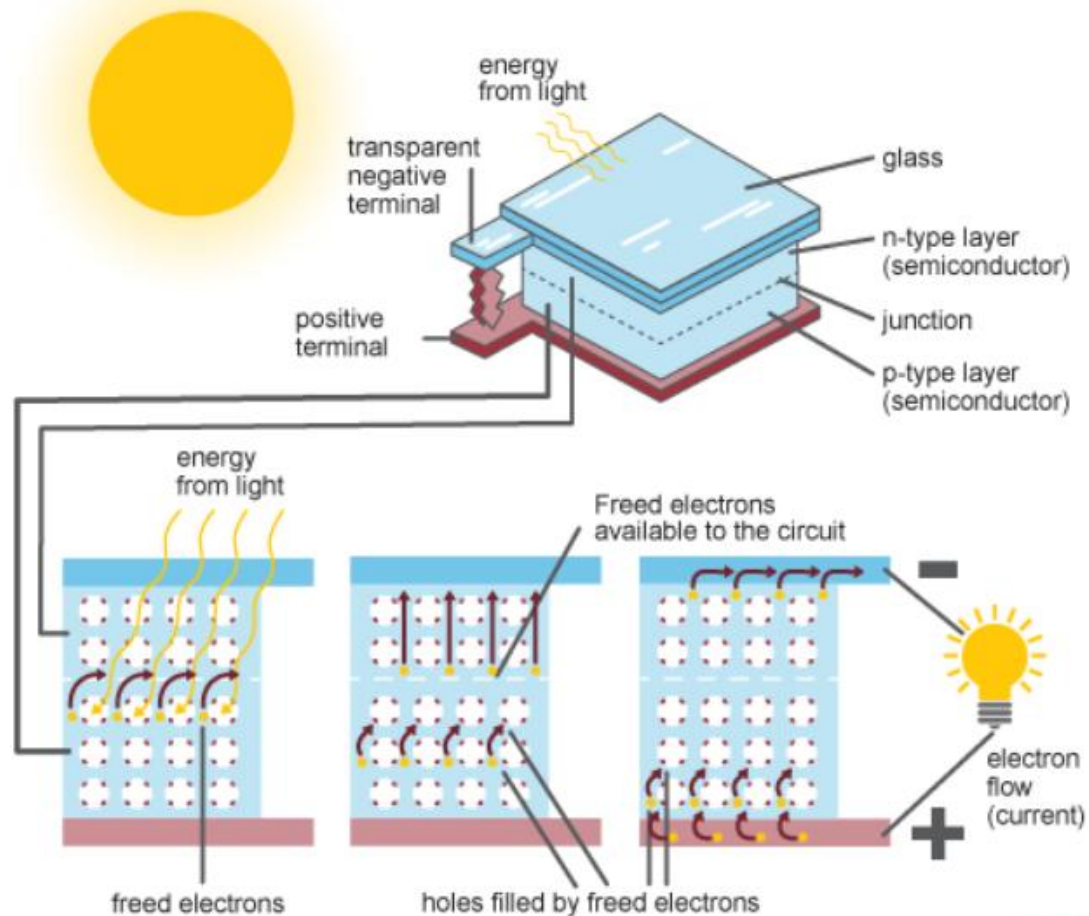
Figure 3.4 Photovoltaic Cell Diagram
