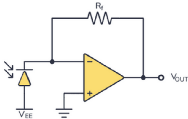
Figure 3.13 Photodiode Light Sensing Circuit [34]
