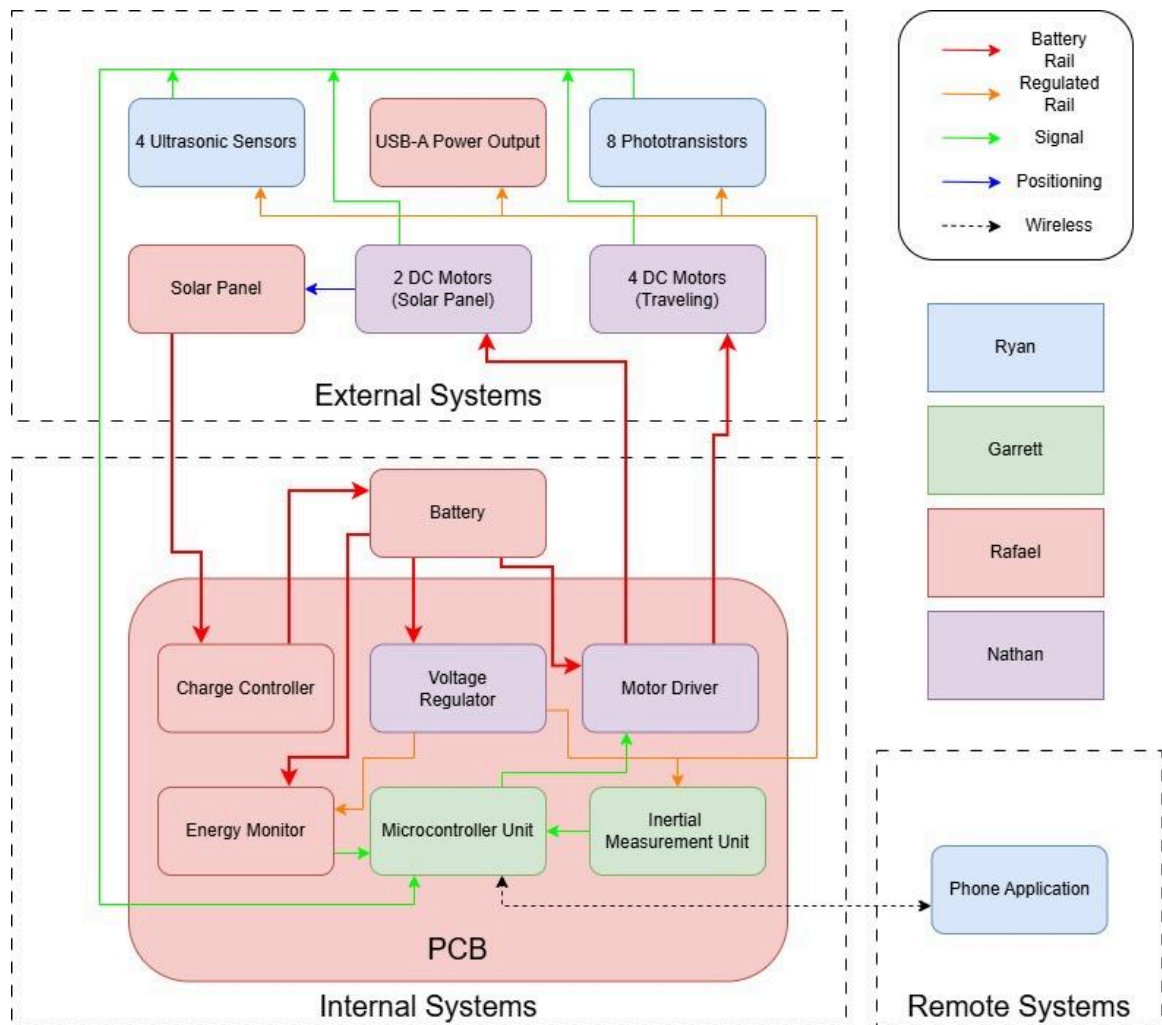
SOLARIS Block Diagram
