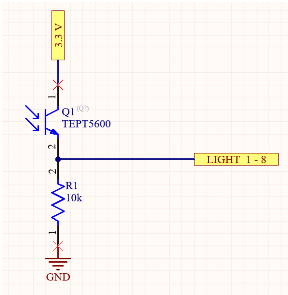
Figure 6.2 Light Sensor Schematic
