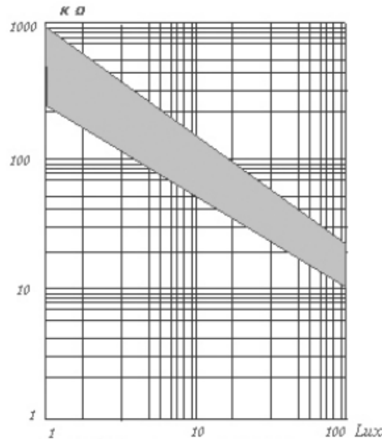
Figure 3.11 LDR Non linear relationship between LUX and Resistance [32]
