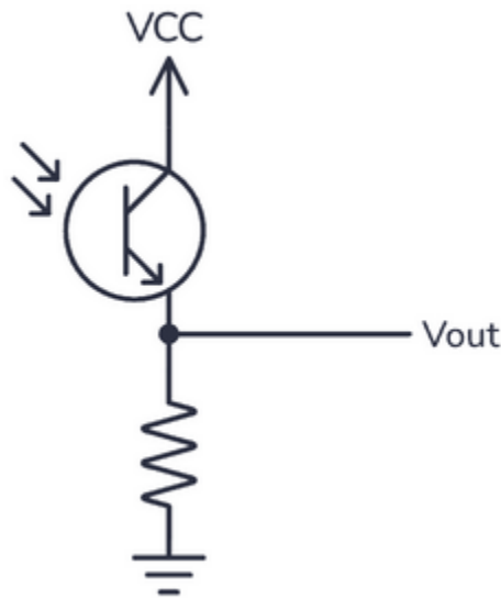
Figure 3.12 Phototransistor Light Sensing Circuit [33]
