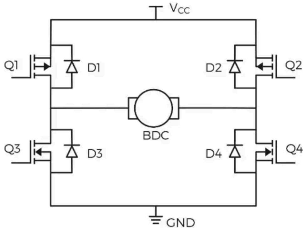
Figure 3.3 H-Bridge Topology [83]
