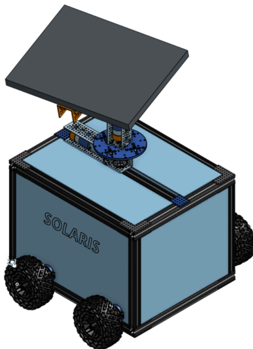
Figure 6.6 SOLARIS Chassis With Covers
