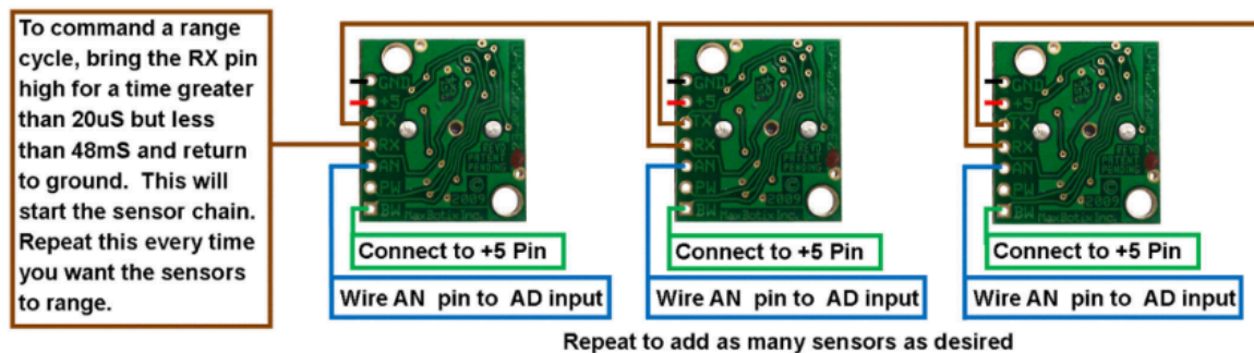
Figure 3.19. MB1020-000 Sensor Chaining Diagram [56]
