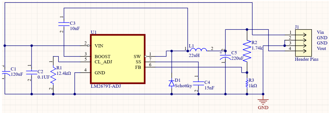
Figure 6.3 3.3V Regulator Schematic
