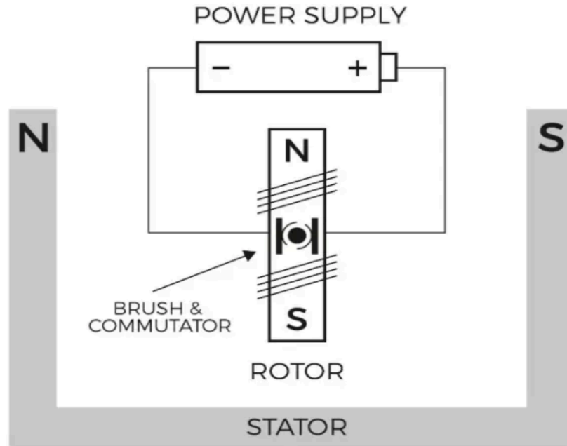
Figure 3.2 Two-pole DC Motor Model [83]
