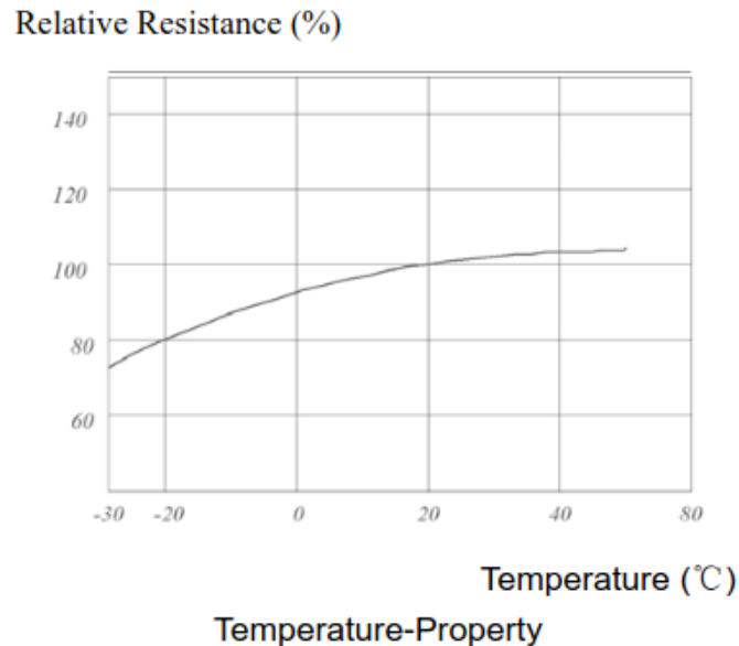
Figure 3.10 LDR Resistance vs Temp [32]
