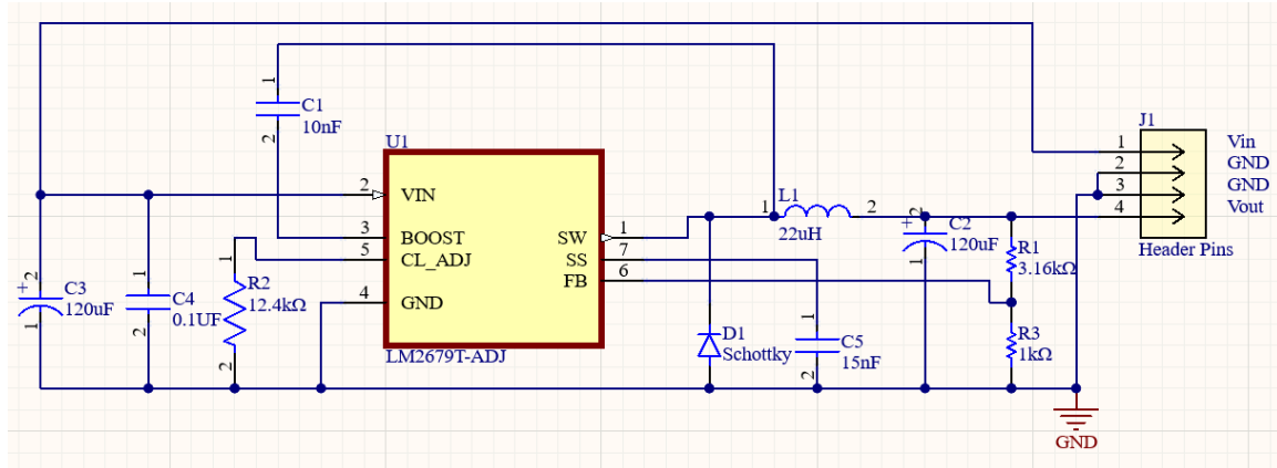
Figure 6.4 5V Regulator Schematic
