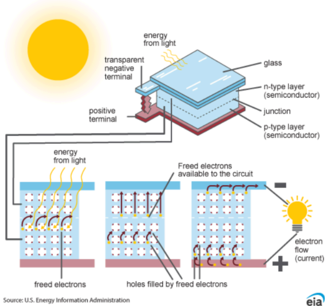
Figure 3.4 Photovoltaic Cell Diagram [43]
