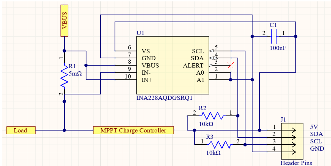
Figure 6.1 Energy Monitor Schematic
