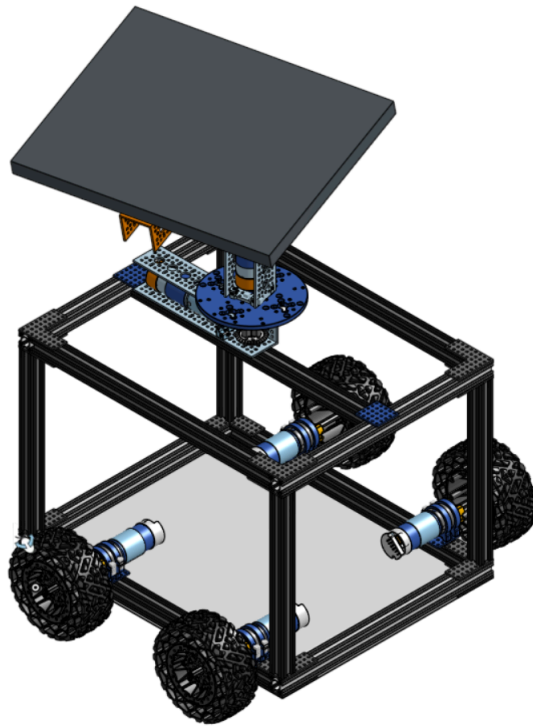
Figure 6.5 SOLARIS Chassis Without Covers
