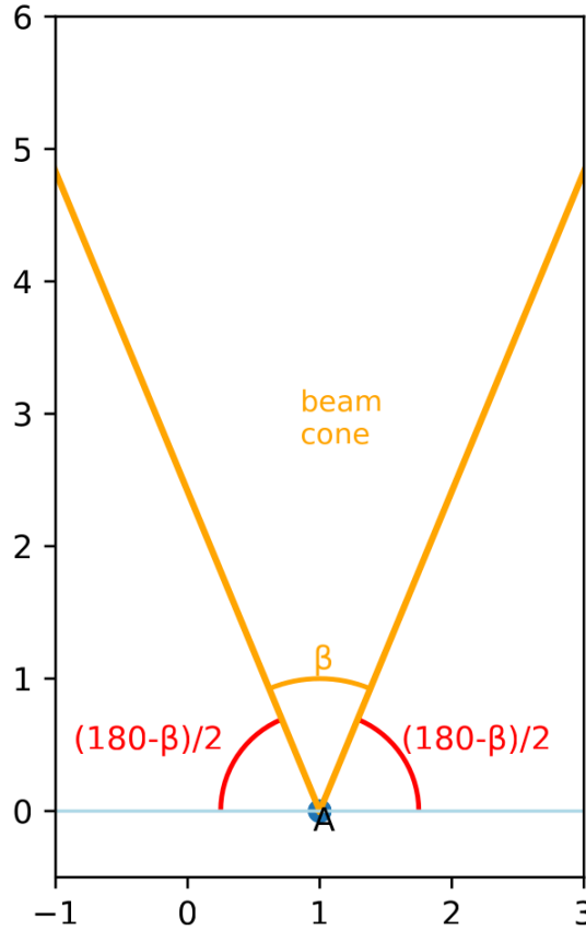
Figure 3.16 One Ultrasonic Sensor Flush With X-Axis
