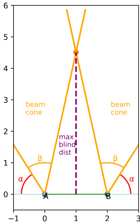
Figure 3.15 Two Ultrasonic Sensor Beam Cone Coverage
