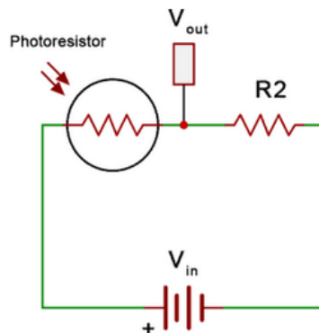
Figure 3.9 LDR Light Sensing Circuit [31]
