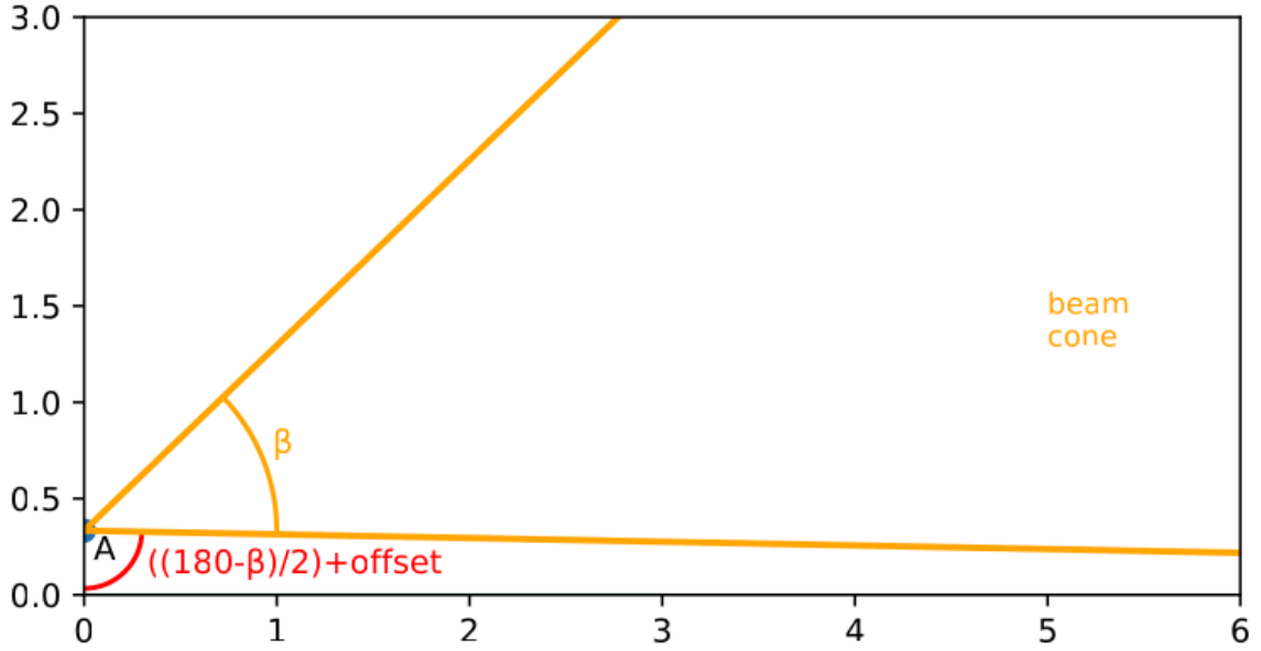
Figure 3.18. Ultrasonic Sensor Angle Pointing Towards the Ground
