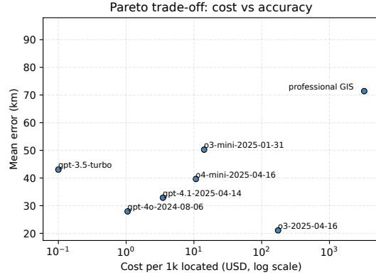
Figure 5: Cost-Accuracy Tradeoff
