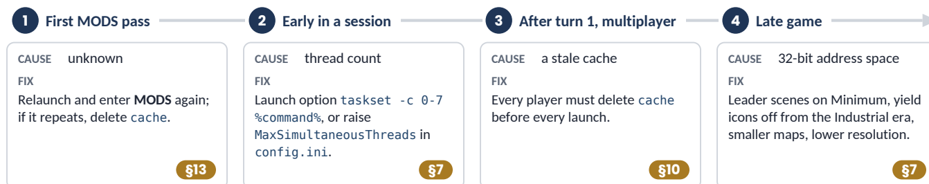
Figure 5 · Crash triage by when the crash happens.
