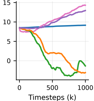
HalfCheetah v5
