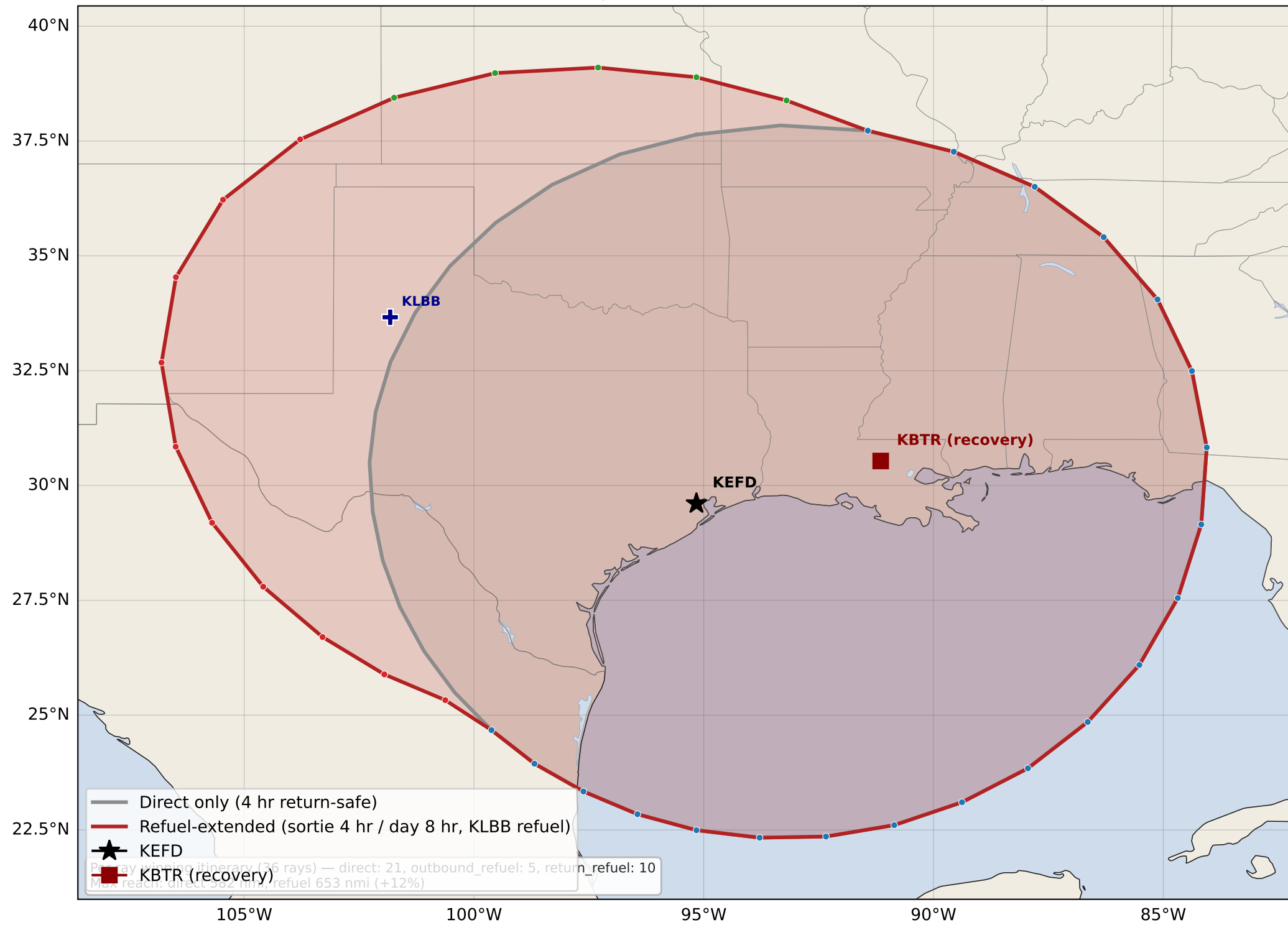
B-200 wind-aware reachability — direct vs refuel-extended (30 kt westerly)
