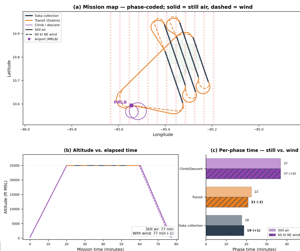
Figure 2: Wind-aware mission planning for the same Rincón de la Vieja survey using a King Air B-200. (a) Mission map; solid lines are still-air Dubins arcs and dashed lines are trochoidal arcs under a 60 kt northeasterly wind, both color-coded by phase. (b) Altitude vs. elapsed mission time, both conditions overlaid. (c) Per-phase time totals (still vs. wind) for climb/descent, transit, and data collection, with absolute deltas annotated. Wind redistributes time across phases — transit arcs distort while data-collection legs see crab-corrected groundspeed effects — even when total mission time changes only modestly, an effect that propagates into fuel planning and airspace coordination.
