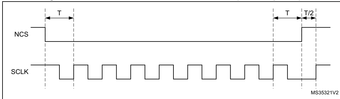
Figure 67. NCS when CKMODE = 1 in DDR mode ( T = \text{CLK period} )
