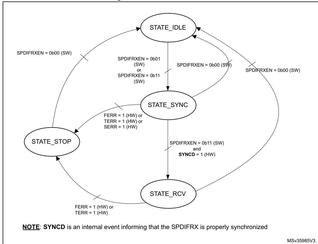
Figure 347. SPDIFRX states
