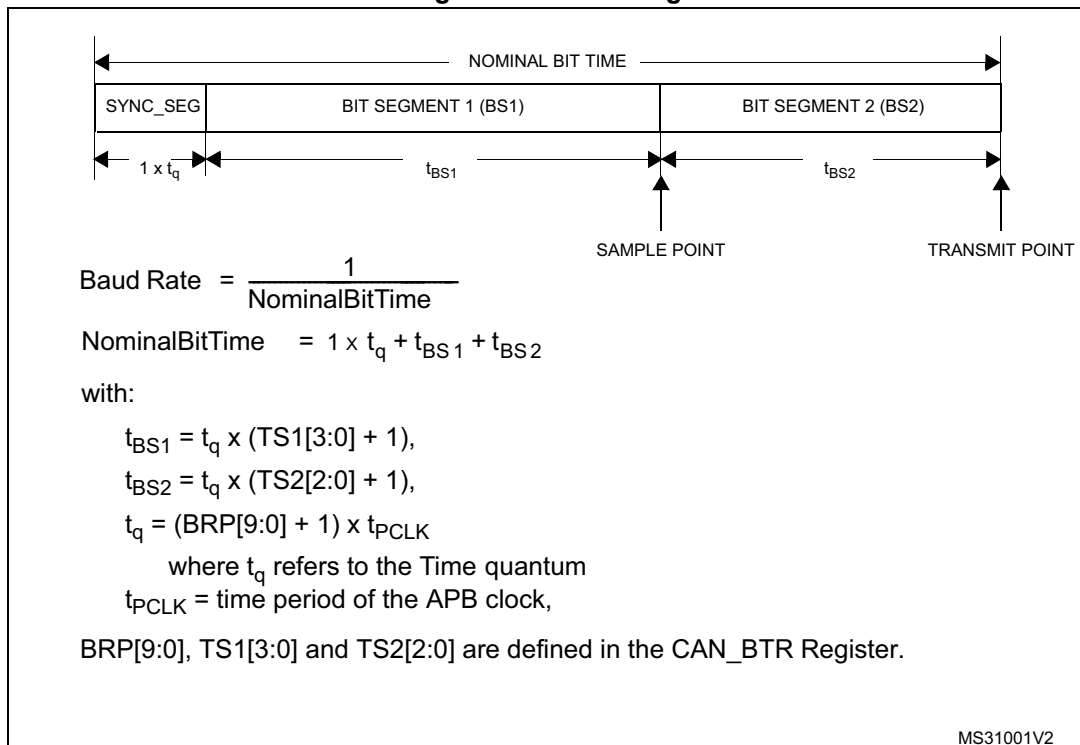
Figure 395. Bit timing
