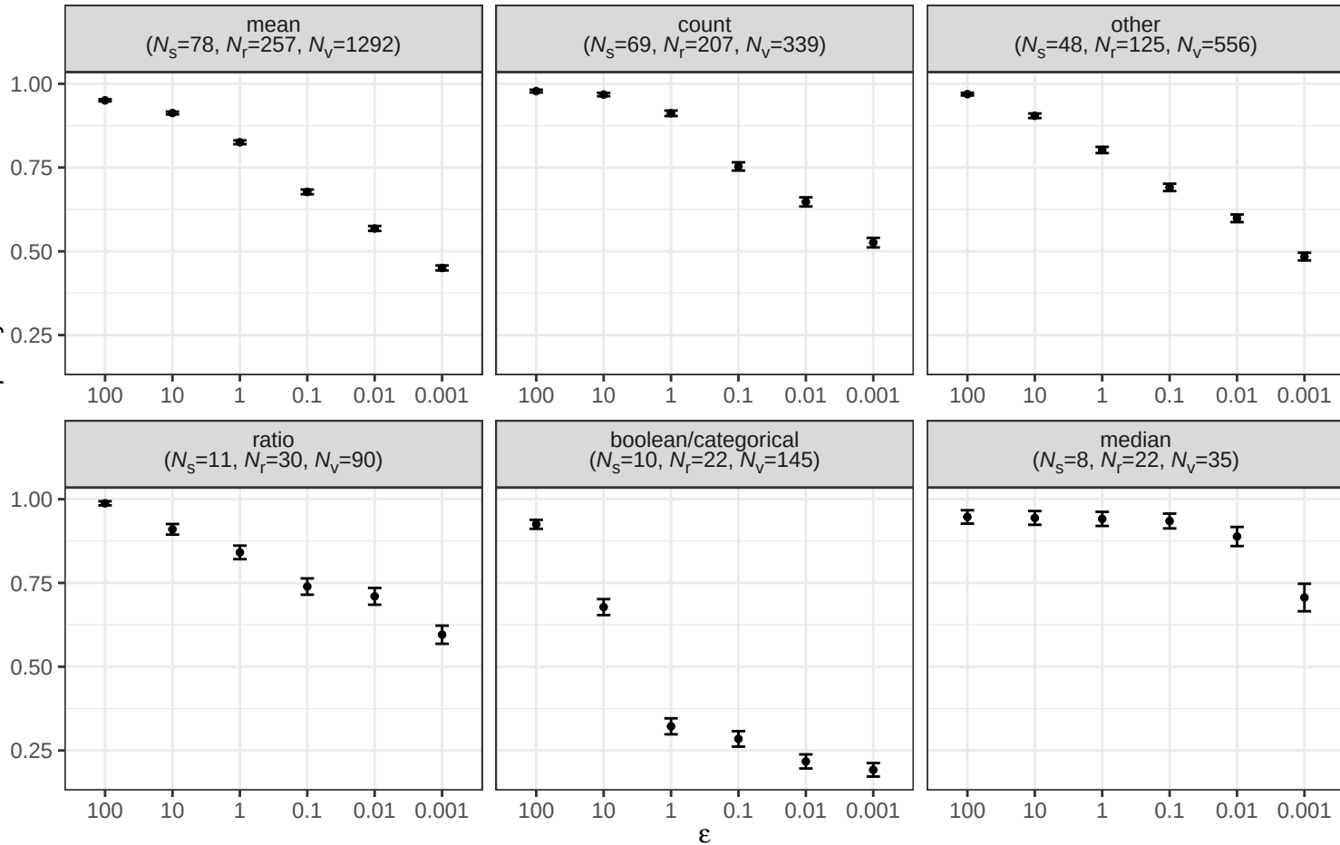
Rate of strict parity
