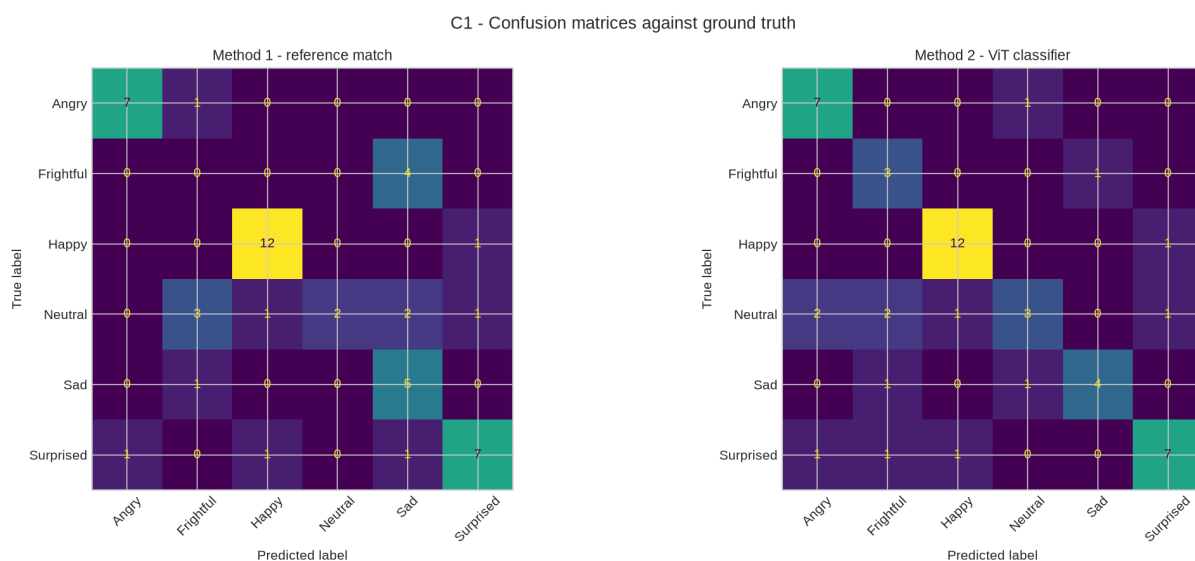
Figure 18: C1 – Confusion matrices for both methods against ground truth.
