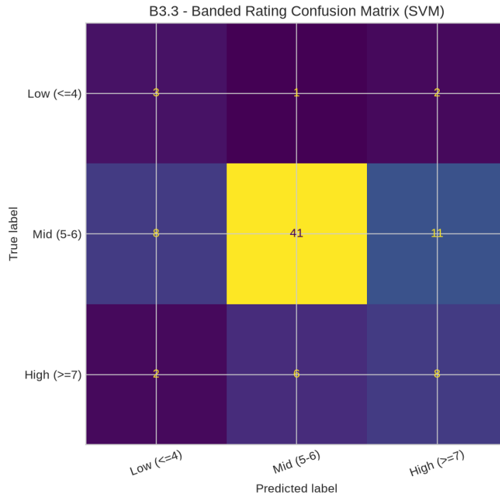
Figure 14: B3.3 – Confusion matrix on the banded target. The Mid band is recovered well; the minority bands are separated far better than any individual rare grade was.
