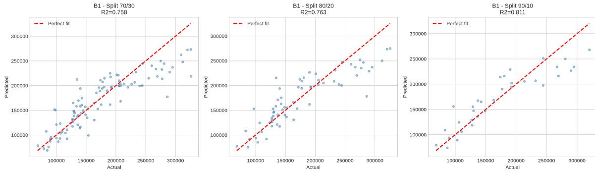
Figure 9: B1 – Predicted against actual price for each split.
