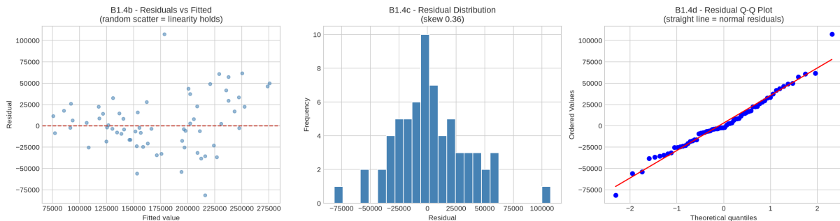
Figure 10: B1 – Residual diagnostics: residuals against fitted values, their distribution, and a normal Q-Q plot.
