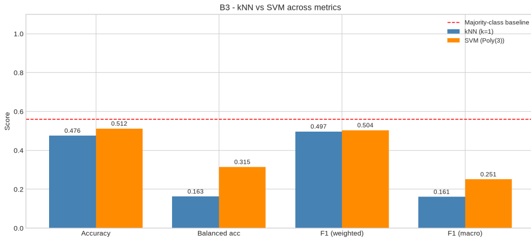
Figure 13: B3 – kNN against SVM across four metrics, with the majority-class baseline.
