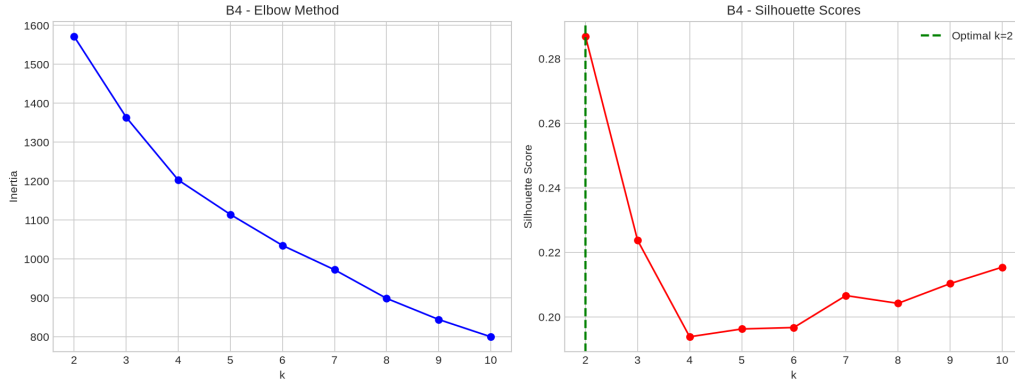
Figure 15: B4 – Elbow and silhouette curves.
