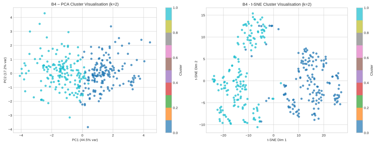
Figure 16: B4 – Clusters under PCA (left) and t-SNE (right).
