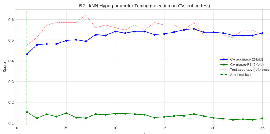
Figure 12: B2 – k-NN tuning. Selection uses the cross-validated curve, not the test curve.
