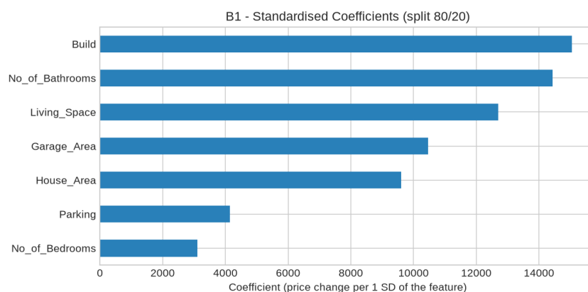
Figure 11: B1 – Standardised feature coefficients.
