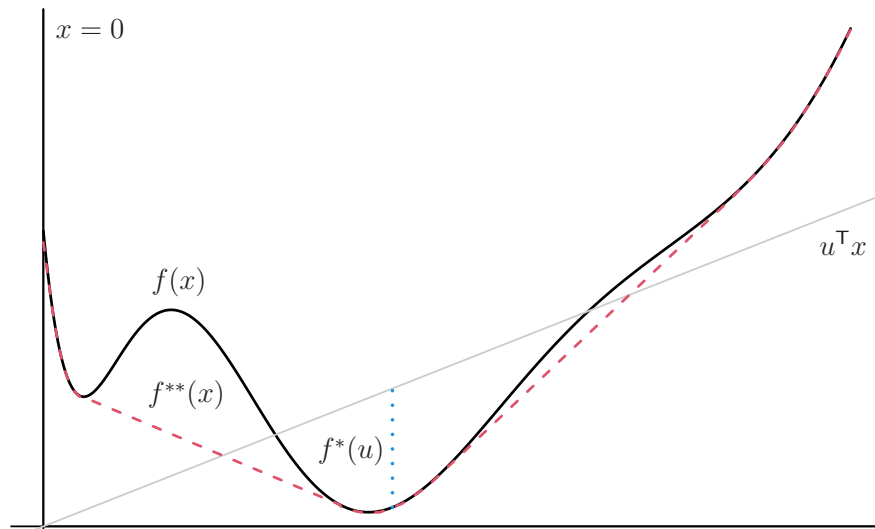
Figure 10.1. The conjugate f^* evaluated at u is the maximum gap between a linear function with slope u and f , illustrated by the dotted line. The double conjugate f^{**} is the pointwise supremum of all affine minorants to f (equivalently, the greatest closed convex minorant to f ), illustrated by the dashed line.
