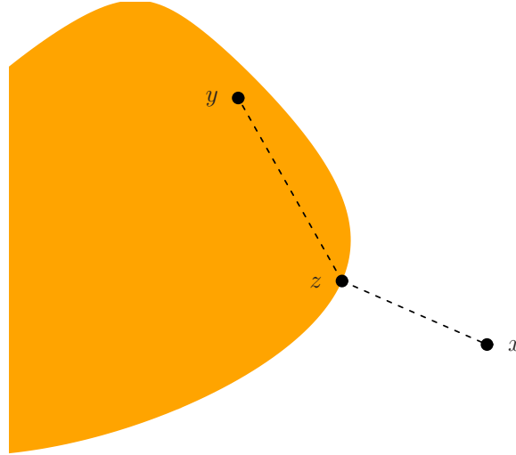
Figure 2.1. Illustration of the variational inequality determining the optimality of the projection z of a point x onto a convex set. The angle between the line segments xz and yz must be at least a right angle (at least 90^\circ ), for any other point y in the set.
