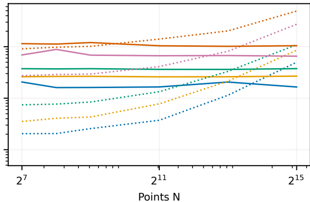
Halton: fresh scrambling + sampling
