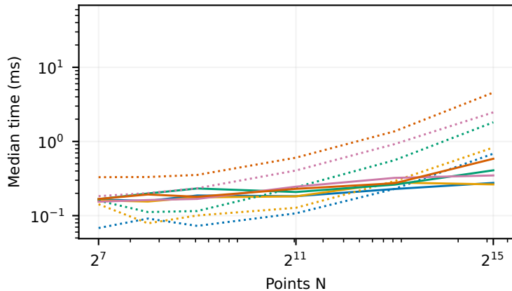
Sobol: fresh scrambling + sampling
