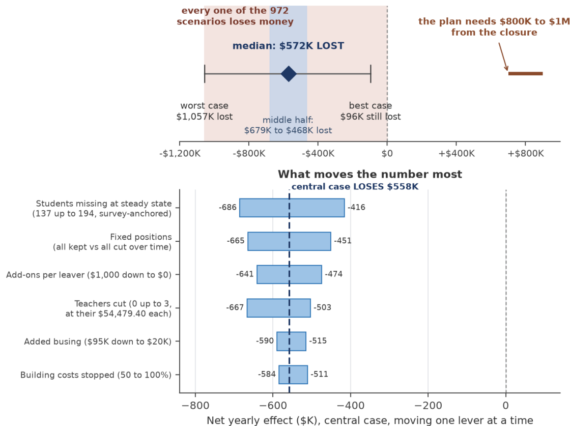
Figure 5. The honest range. Top: the net yearly effect of closure across all 972 combinations of the six sourced inputs, from losing $1,057,265 to still losing $95,750, with the middle half of weighted scenarios between a $679,361 and a $467,862 loss and the median at a $571,883 loss. The plan's own $800,000 to $1,000,000 requirement lies entirely outside the defensible range. Bottom: how far each input moves the central case by itself. Inputs: the district's own response worksheet and staffing appendix (Appendix A and A.1), its capacity appendix, its KDE filings, the federal attendance-zone map, and the exit routes open under HB 563, homeschooling, and the statewide virtual academy; every lever and formula is in the workbook's Closure_Model tab.
