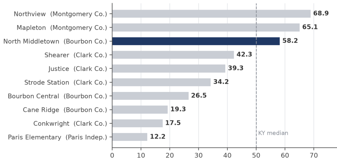
Figure 7. SchoolDigger's normalized 0-100 index for 2024-25 across the region's elementary schools, computed from state test data (not KDE's official rating). Only Montgomery County's two elementary schools outscore North Middletown; every elementary in Bourbon County, Clark County, and Paris Independent trails it.
