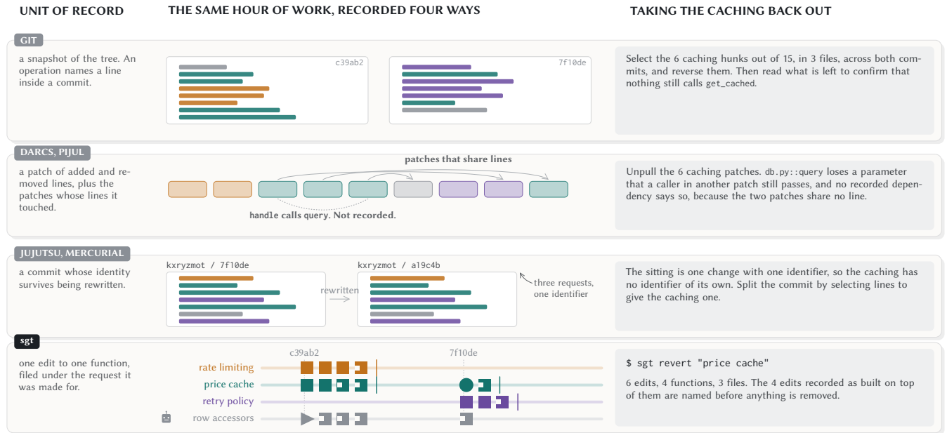
Figure 2: One hour of work with a coding agent, recorded four ways, with the same request removed from each. The unit a system records decides which sets a developer can name. Git and Darcs both bottom out at a line, so removing the caching means selecting lines. Jujutsu and Mercurial add a durable identity above the line, and that identity belongs to a commit, so a squashed session carries one identity for all three requests. sgt records one edit per function together with the request it was made for. The developer supplied that request and never wrote it down.
