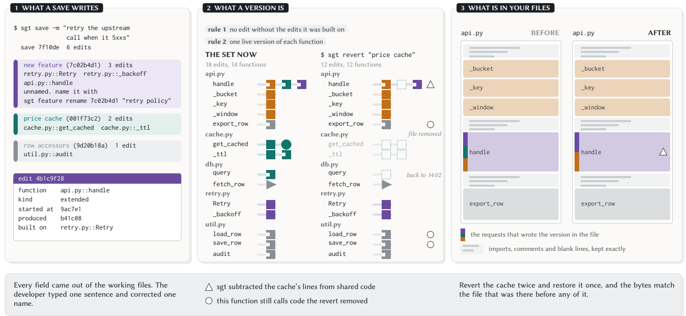
Figure 3: What one save writes down, what a version is, and where the bytes in a file come from. A save writes one record per changed function under a guess at the request it served, and one command corrects the guess (1). A version is the set of those records, so taking out the price cache subtracts six records from eighteen (2). The files are rebuilt from that set with the text between functions kept exactly (3). Where the cache's lines had to be subtracted from a function later work also edited, the developer's test suite decides whether the result stands.
