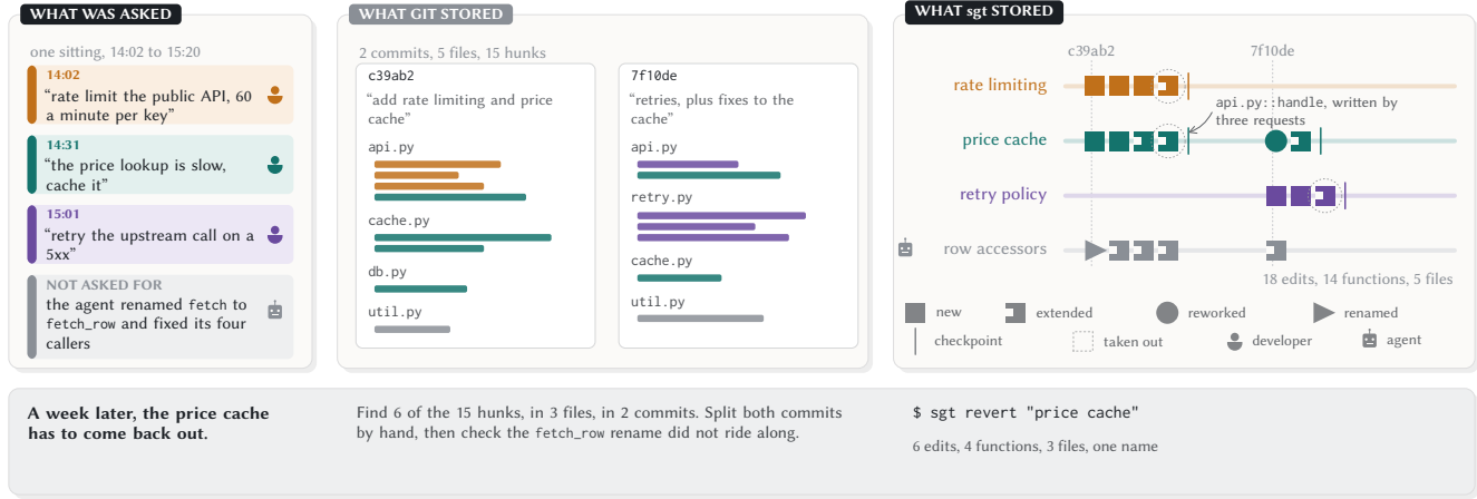
Figure 1: One hour with a coding agent, recorded two ways. The developer stated three requests and the agent made a fourth change nobody asked for. Git stored two commits whose fifteen hunks interleave all four, and the colours in that panel are ours, since git holds no record of which request produced which hunk. sgt stored one edit per changed function under the request it came from, so the caching is six edits with a name.
