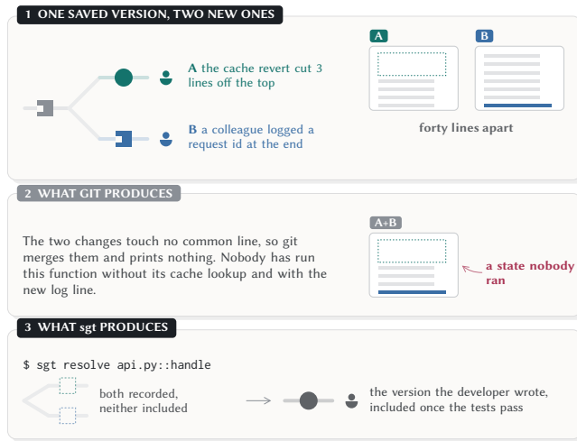
Figure 4: Two people change api.py::handle from the same saved version, one cutting three lines from the top of it and one adding a line forty lines below. Git merges the two and prints nothing, and nobody has run the function in the state the merge produces. sgt records both versions, includes neither, and names the function. Of everything sgt refuses, only this refusal can stop work that would have been correct.
