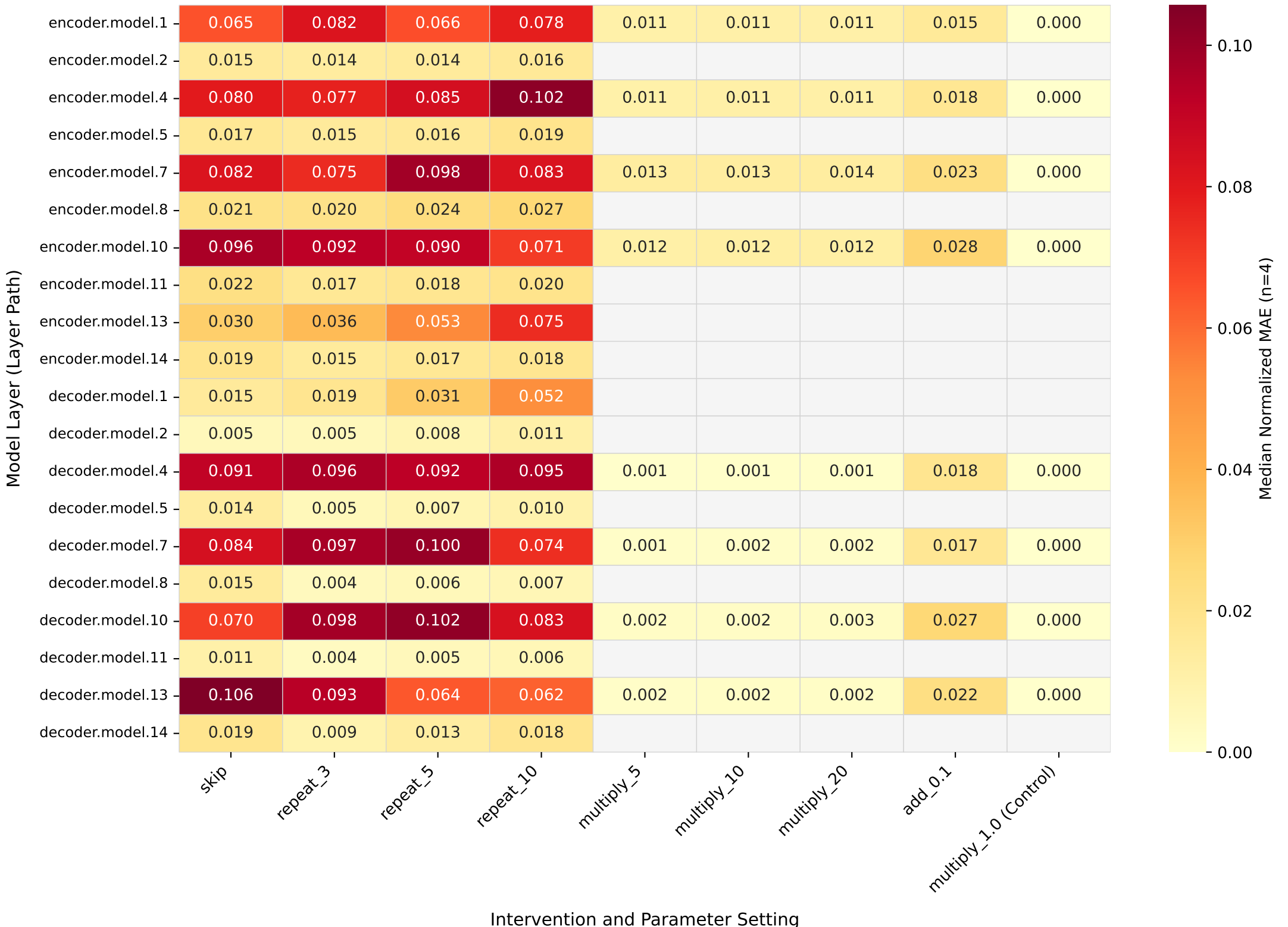
Intervention Heatmap: Median Normalized MAE EnCodec (48 kHz) | Aggregated across four recordings
