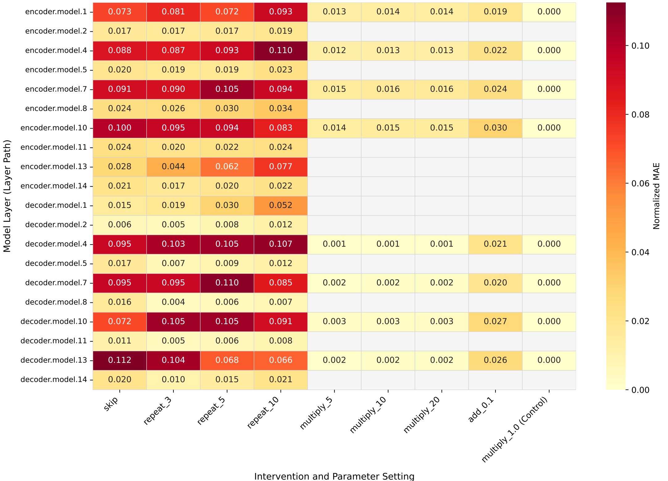
Intervention Heatmap for Stimulus: AmenBreak.wav EnCodec (48 kHz)
