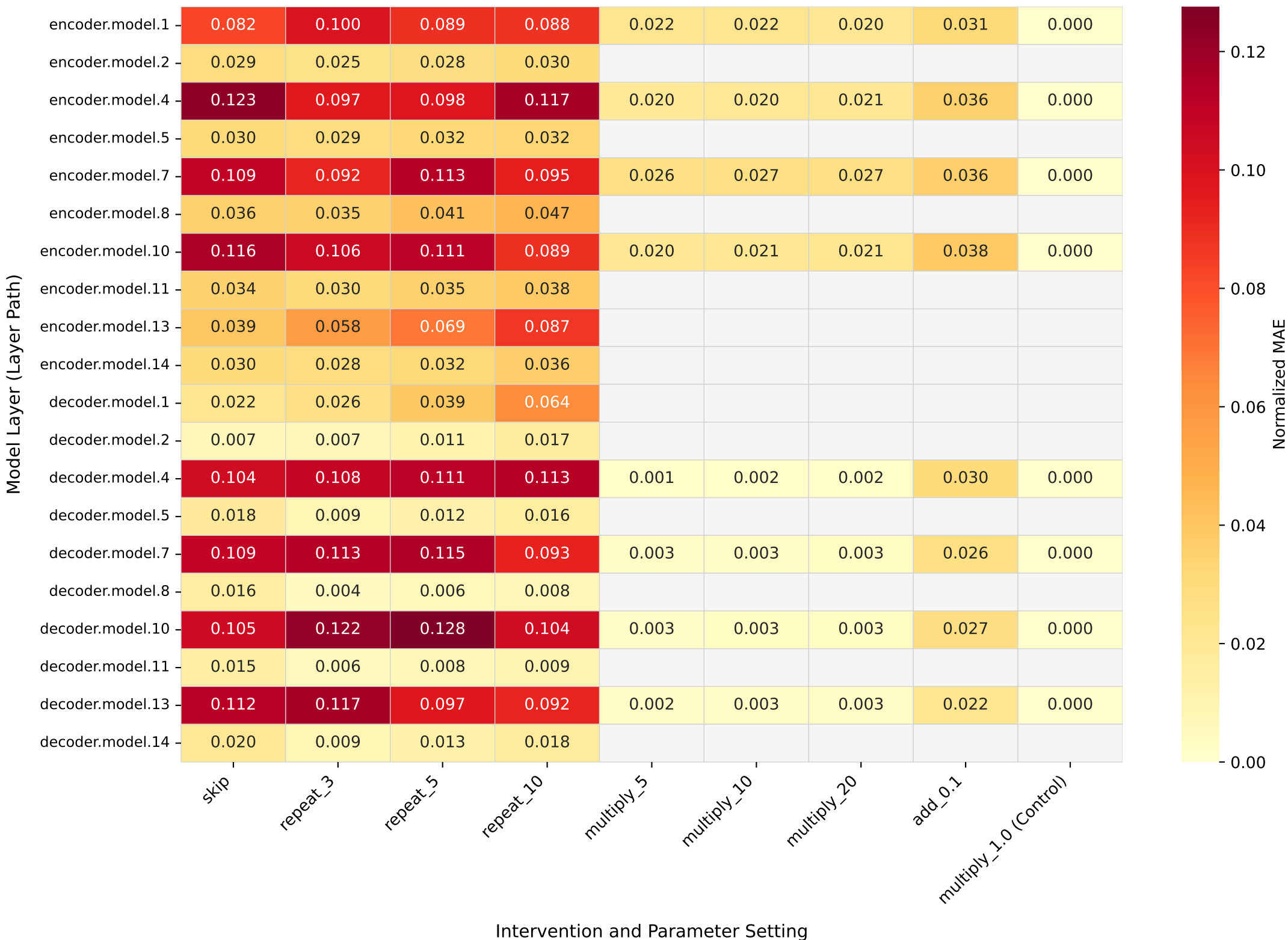
Intervention Heatmap for Stimulus: GLM.wav EnCodec (48 kHz)
