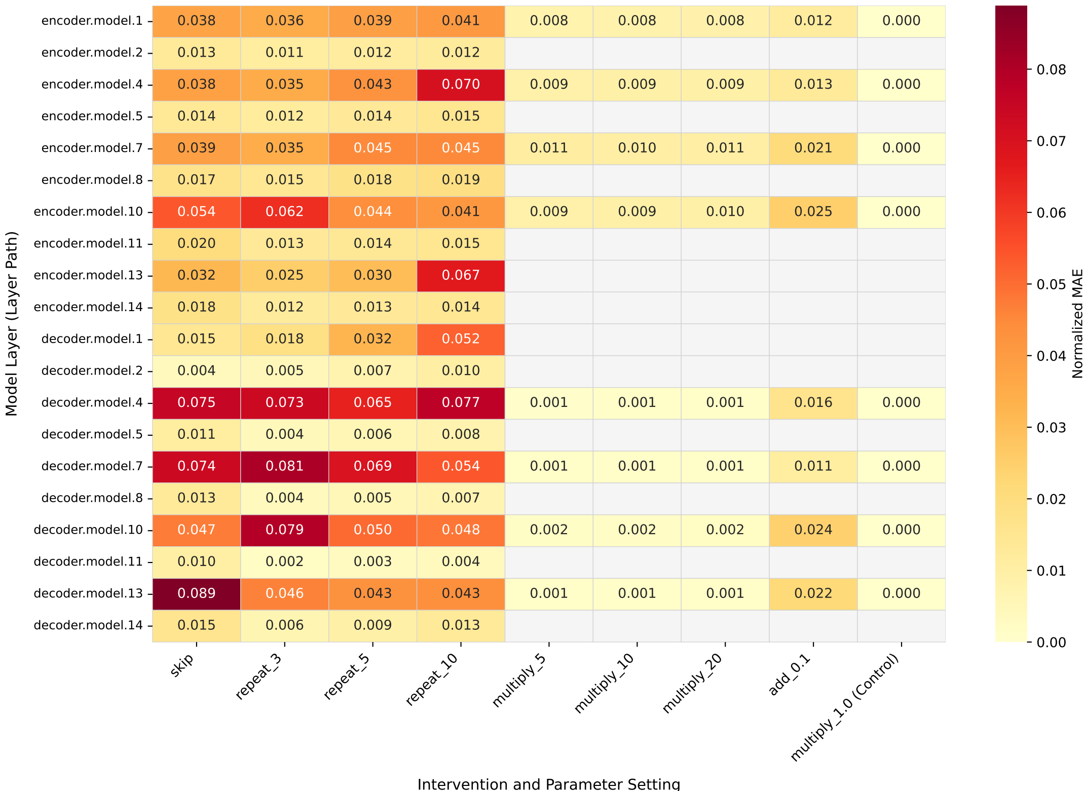
Intervention Heatmap for Stimulus: tof.wav EnCodec (48 kHz)
