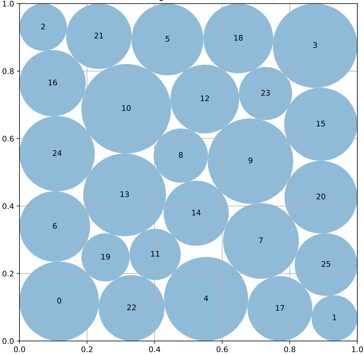
Circle Packing (n=26, sum=2.626293)
