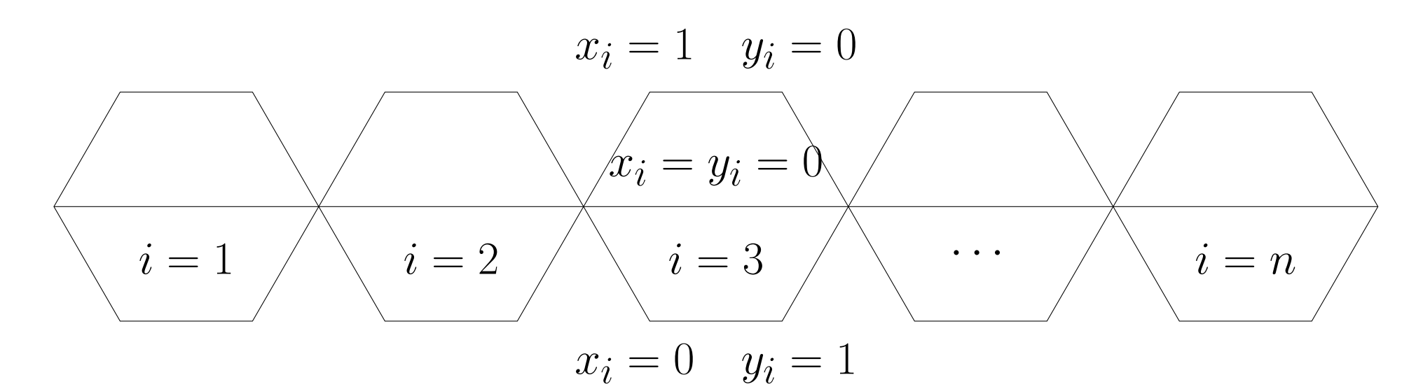
Figure 8. Chain of Disjoint Gadgets
