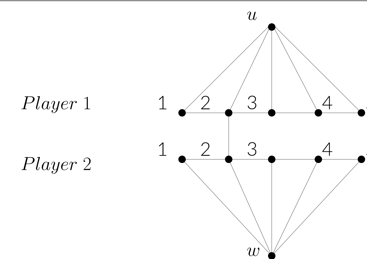
Figure 8. Chain of Disjoint Gadgets
