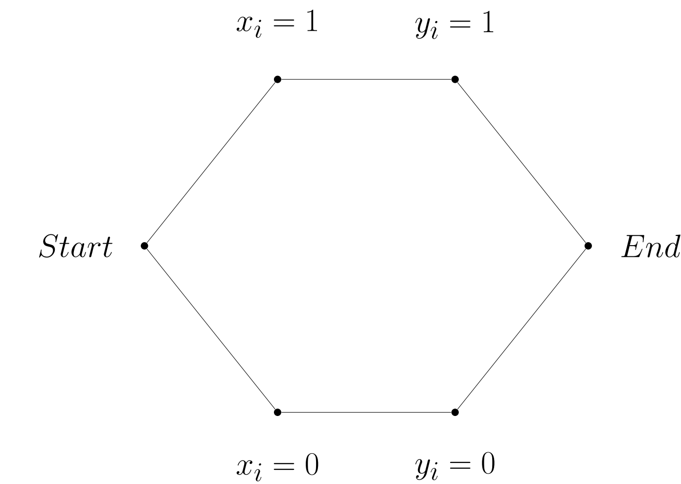
Figure 6. Gadget for proving equality Embedding
