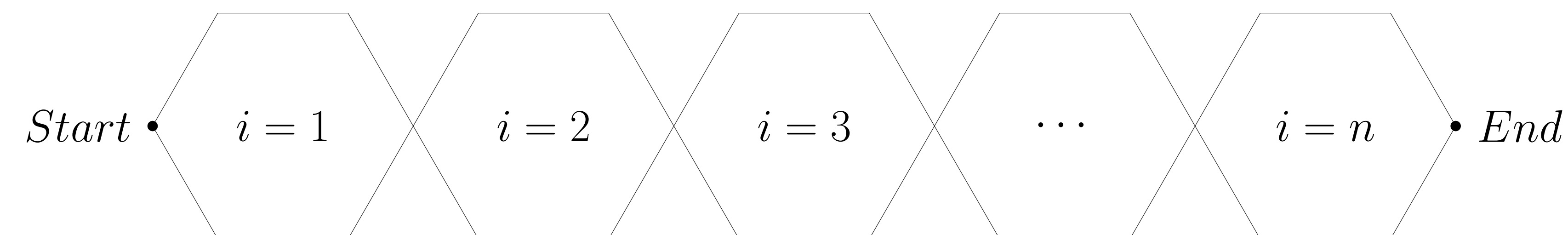
Figure 7. Chain of Equality Gadgets
