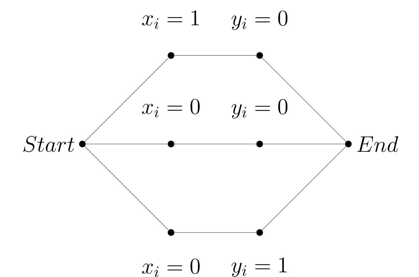
Figure 9. Disjointness gadget. A path Start to End only exists if either x_i = 0 or y_i = 0 .
