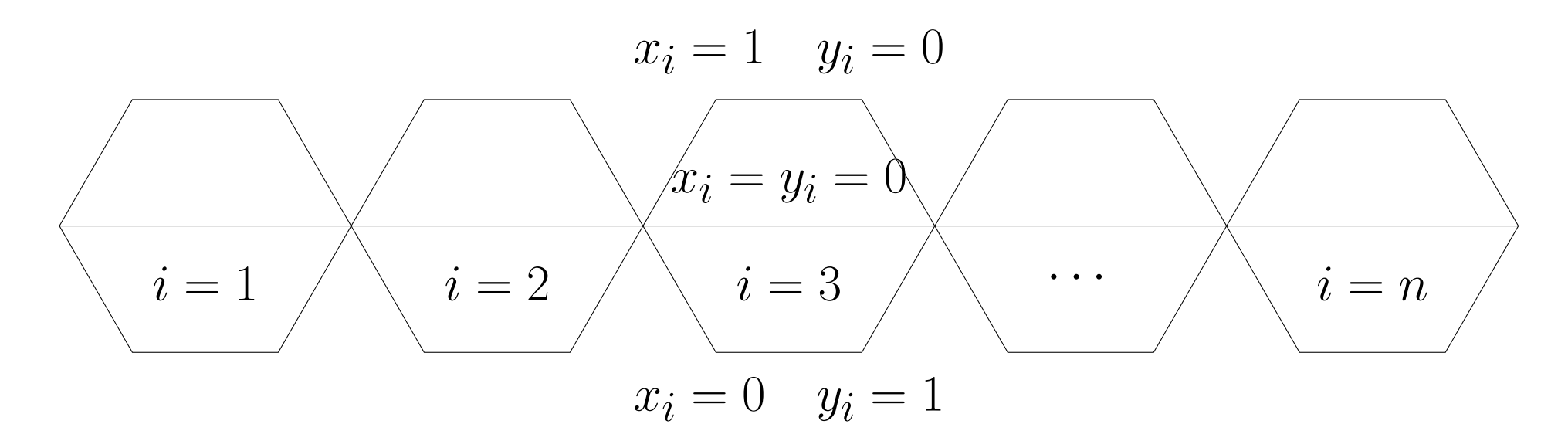
Figure 8. Chain of Disjoint Gadgets
