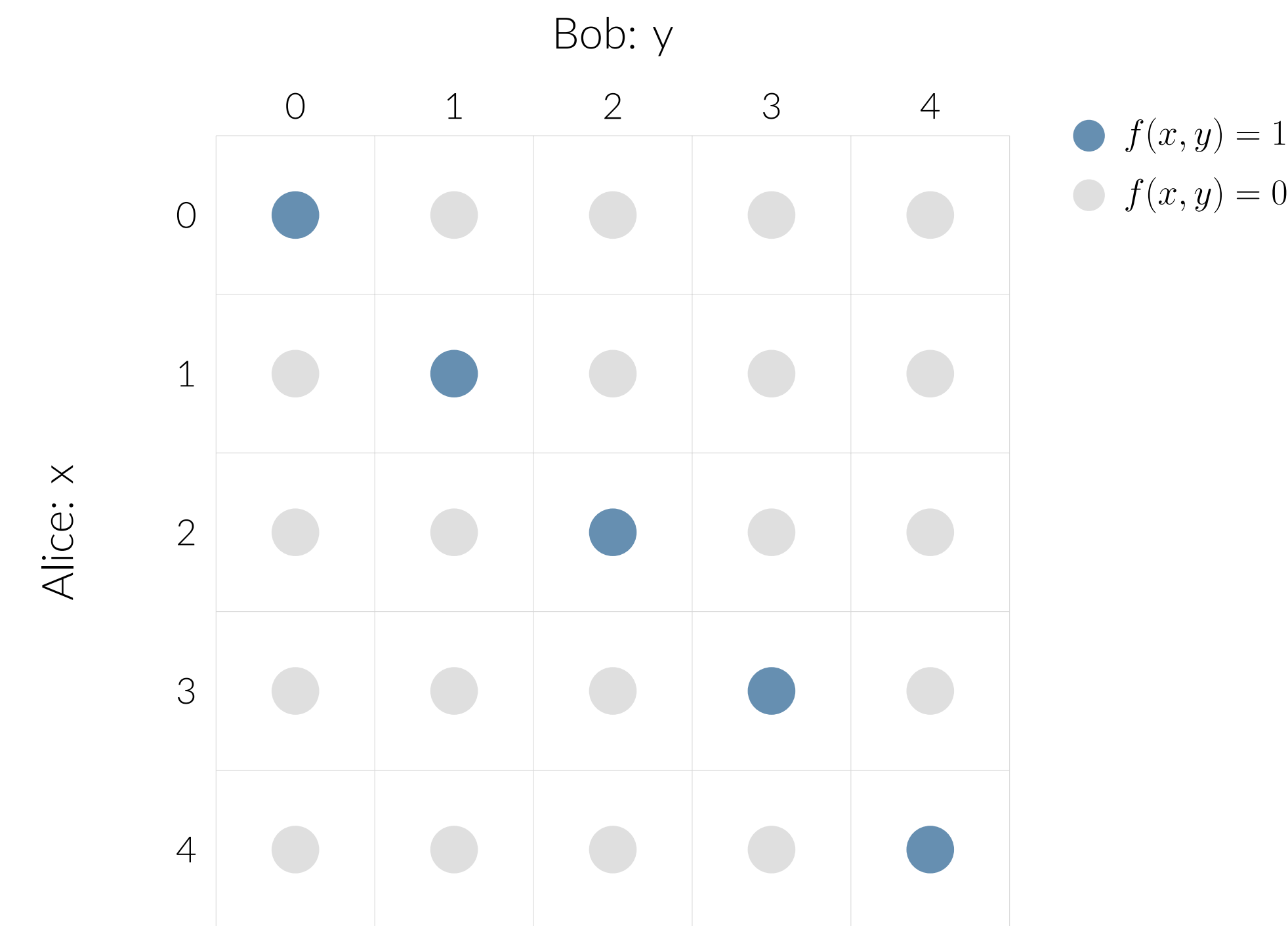
Figure 3. Communication matrix for Equality
