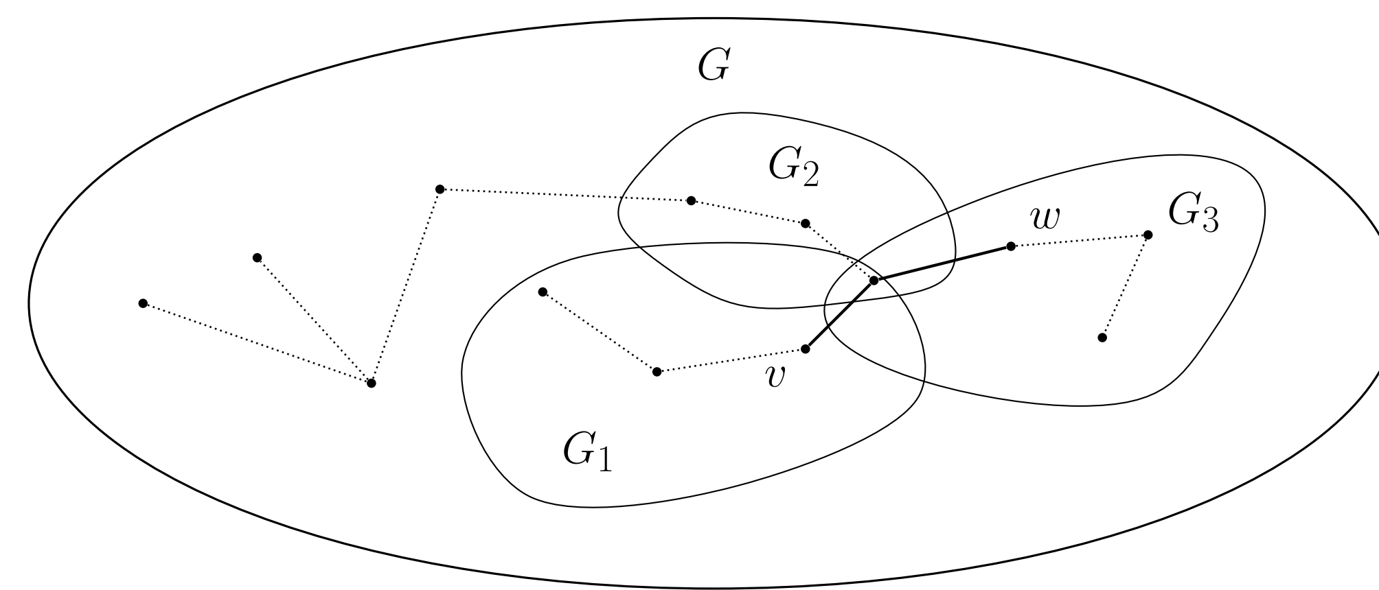
Figure 4. TRAV example where a valid path from v to w is shown in bold.
