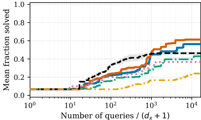
(a) Data profile, \tau = 10^{-1}
