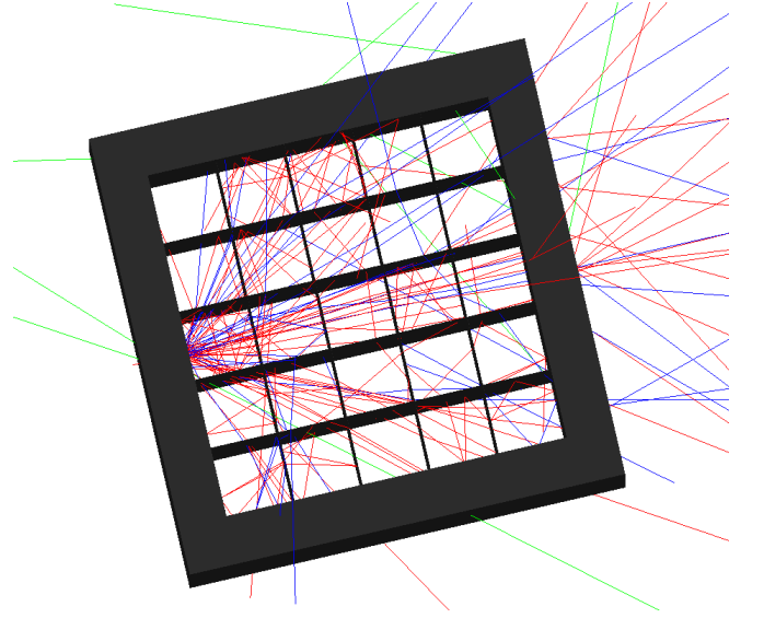
FIG. 12: Render of the moderator modeled off of the Slow Positron Facility at KEK. Electrons (red) hit the target from the leftmost edge and the resulting positrons (blue) stop in the mesh.
