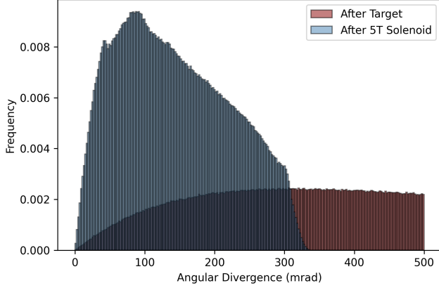
FIG. 3: Angular divergence histogram of positrons before and after passing through the adiabatic matching device. The AMD reduces the spread of nearly all particles to under 300 mrad.
