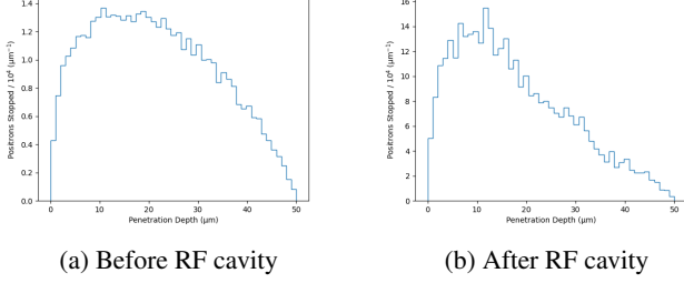
FIG. 11: Stopping distributions of positrons at normal incidence, using the energy values from Fig. 2.
