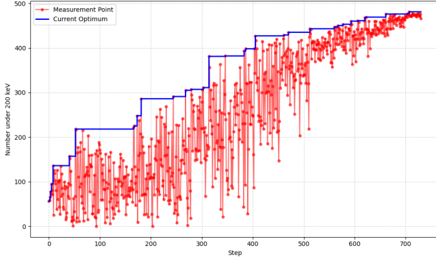
FIG. 9: The simulated annealing algorithm used to tune RF cavity. Here, the goal was to optimize the number of positrons under 200 keV, which are the most likely to stop in the moderator. Different goals were used to produce the greatest yield in each moderator.
