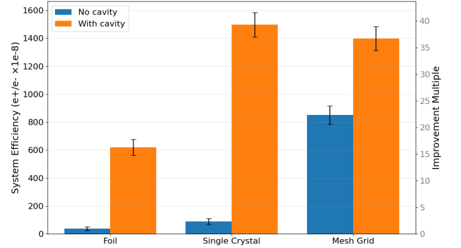
FIG. 13: System efficiency of various moderator geometries, with and without the AMD and RF cavity. The right axis shows the improvement multiple in comparison to the foil moderator without a cavity.
