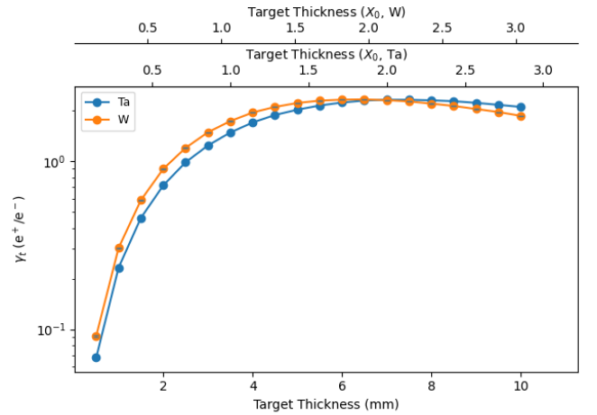
FIG. 1: Positron yield \gamma_t as a function of target thickness (shown in both millimeters and radiation lengths) for tungsten and tantalum. We use 100 MeV electrons; see 5 for a comparable plot with different electron energies.
