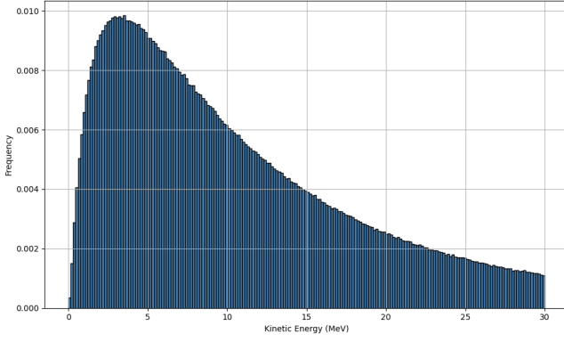
FIG. 2: Energy distribution histogram of positrons emitted in the forward direction from 100 MeV electron collisions with a 7.0 mm tungsten target.
