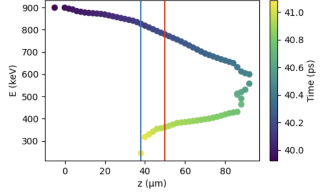
FIG. 7: Particle trace of an incident positron that would contribute to the Makhovian, but passes through a thin foil. The blue line indicates the final stopping point of the particle in a semi-infinite material, while the red line indicates the border of a 50 \mu\text{m} moderator.
