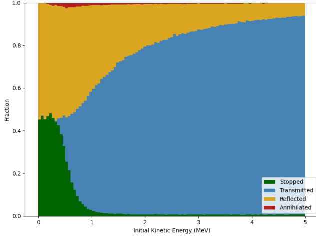
FIG. 6: Outcome of incoming positrons in a 50 \mu\text{m} foil moderator, categorized by initial kinetic energy. Positrons with energy over 1 MeV essentially do not contribute to the moderator yield.
