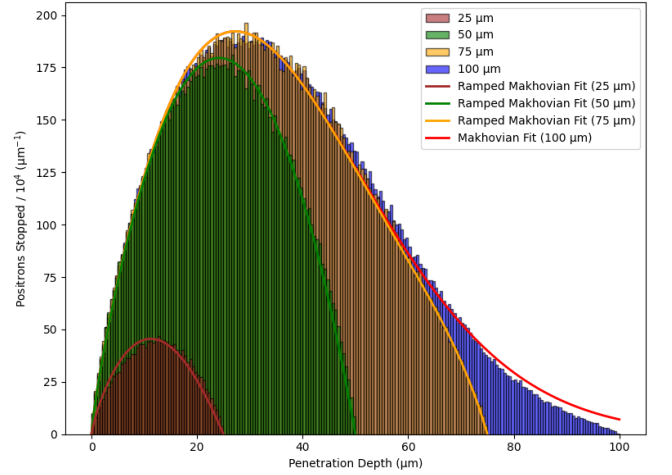
FIG. 8: Simulation (shaded) and ramped Makhovian fits for 500 keV positrons on foils of various thicknesses. The red line is an unramped Makhovian for the 100 \mu\text{m} foil.
