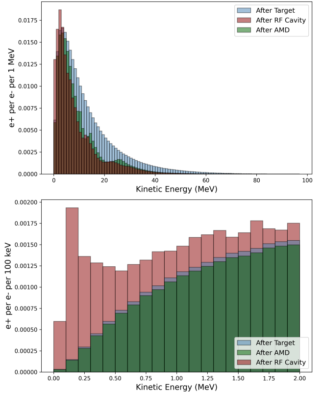
FIG. 10: Resulting energy distribution of positrons before and after passing through the RF cavity. The distribution has been shifted towards lower energies.
