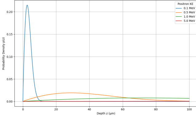
FIG. 5: Makhovian distributions at normal incidence for different positron energies. As expected, lower energy positrons stop much sooner.
