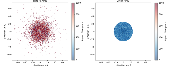
FIG. 4: Cross-section of positron beam a) emitted by the target, and b) after leaving the AMD, colored by angular divergence. The AMD was modeled as a 25mm cylinder.
