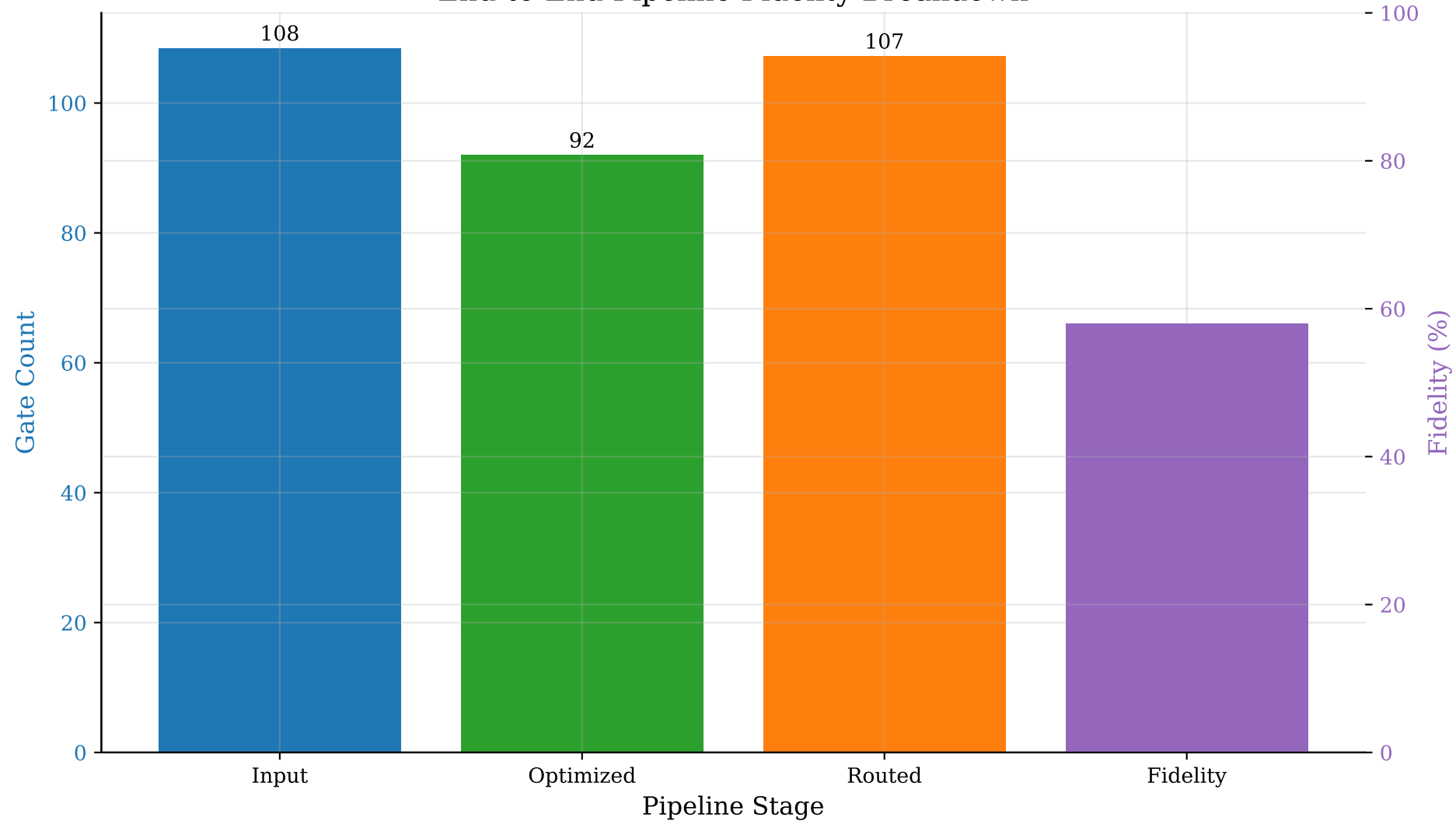
End-to-End Pipeline Fidelity Breakdown
