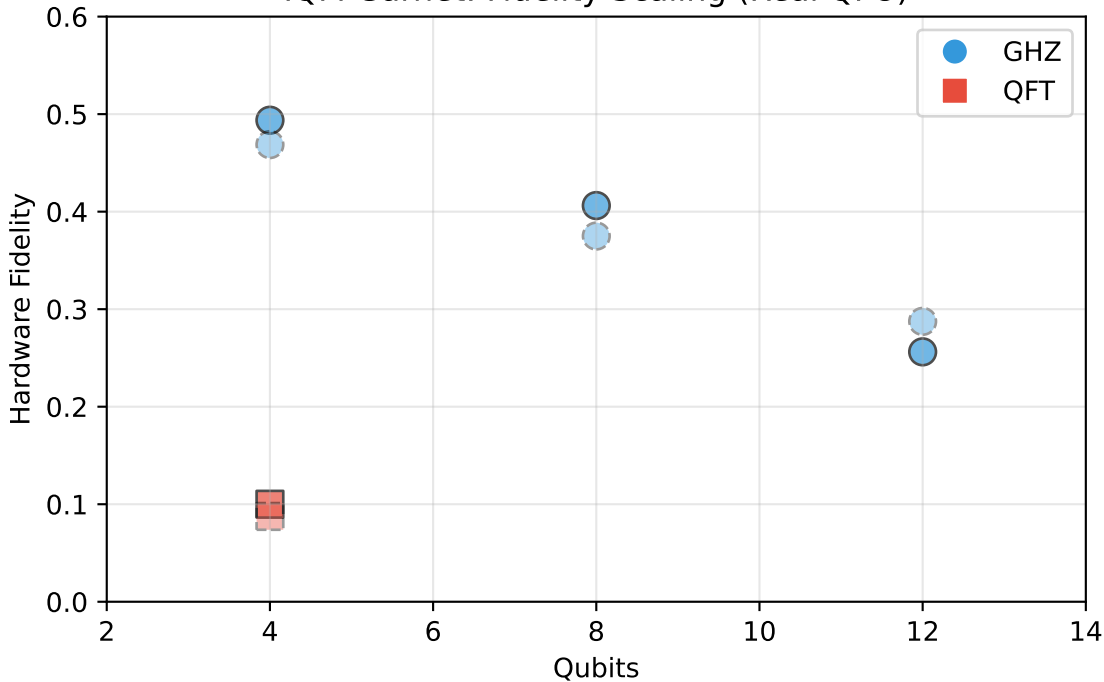
IQM Garnet: Fidelity Scaling (Real QPU)
