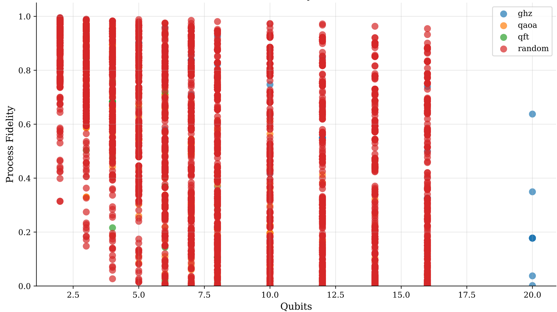
Process Fidelity vs Qubits
