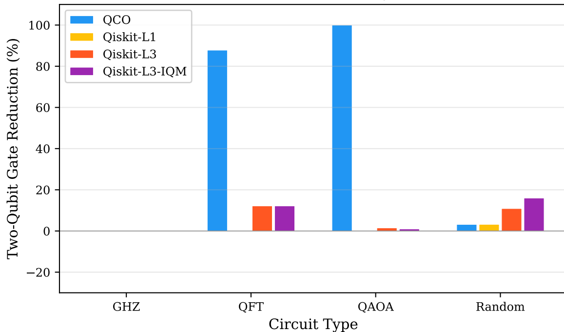
Two-Qubit Gate Reduction by Compiler
