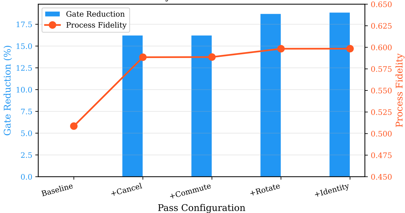
Ablation Study: Cumulative Pass Addition
