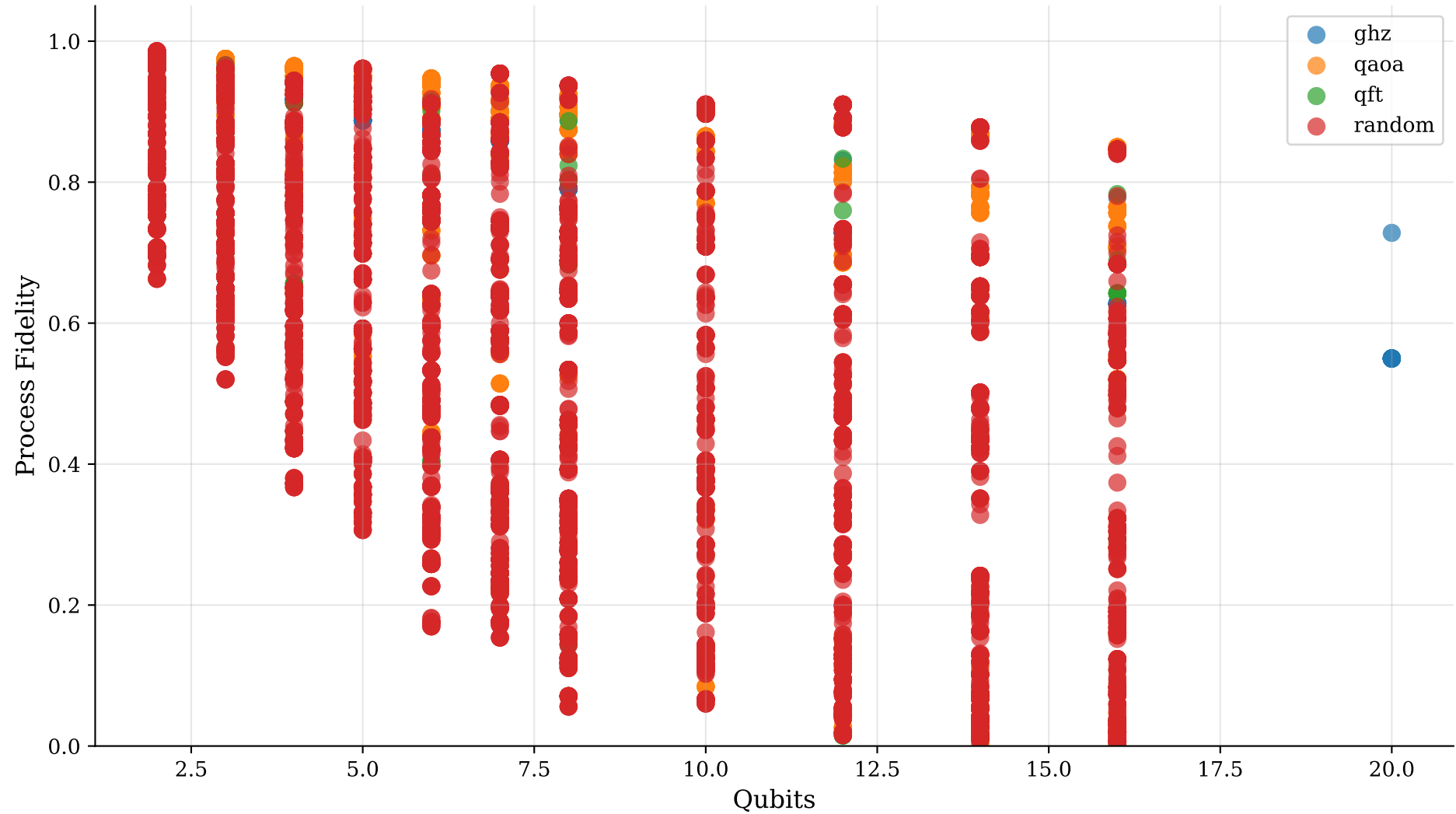
Process Fidelity vs Qubits
